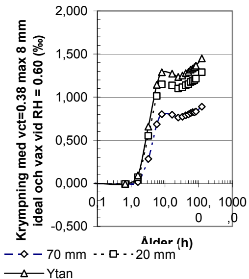
Figur 4.24 – Krympning, vct=0.38 max 8 ideal, vax.
