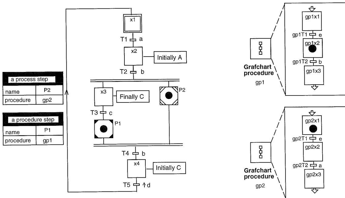
Figure 5.16 A Grafchart.
