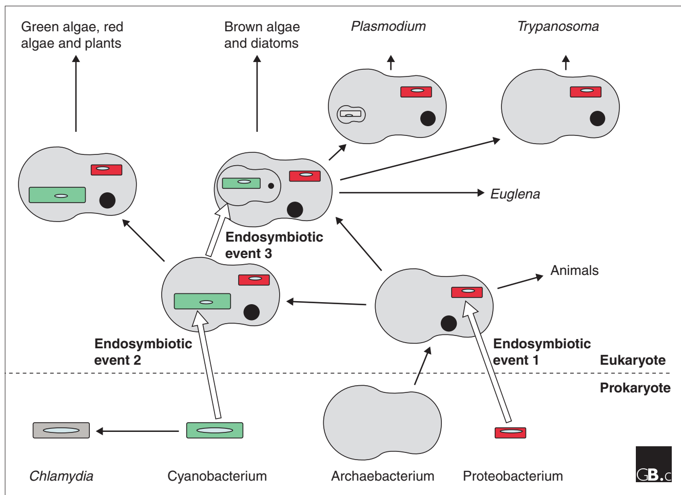
Figure 1 A schematic outline of the acquisition, reduction, and loss of genomes and compartments during evolution. Black arrows indicate evolutionary pathways; white arrows indicate endosymbiotic events in the host cell. Endosymbiotic event 1 occurred at the origin of eukaryotes. The proteobacterial endosymbiont gave rise to mitochondria (the smaller organelles in the bottom part of the diagram). Endosymbiotic event 2 occurred at the origin of plastid-containing cells. Endosymbiotic event 3 represents the secondary and higher-order endosymbioses giving rise to numerous algal phyla, as well as apicomplexans (such as Plasmodium ), which have residual plastids, and to trypanosomes, which have no plastid at all. Black, filled circles indicate nuclei or nucleomorphs; ellipses within organelles indicate bacterially derived genomes, which may be reduced or lost completely. More than one kind of host cell and of endosymbiont is involved in the secondary, and in the higher-order, symbioses. The genome of the Archaeobacterium is not represented in the diagram.
