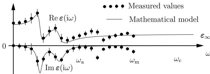
Figure 2.2: Illustration of the range of validity of the constitutive relations. The measured values of the constitutive map \varepsilon are known up to frequency \omega_m , the mathematical model is used for frequencies up to \omega_a , and \omega_c is the upper limit for the use of a continuum model of the medium, respectively.
