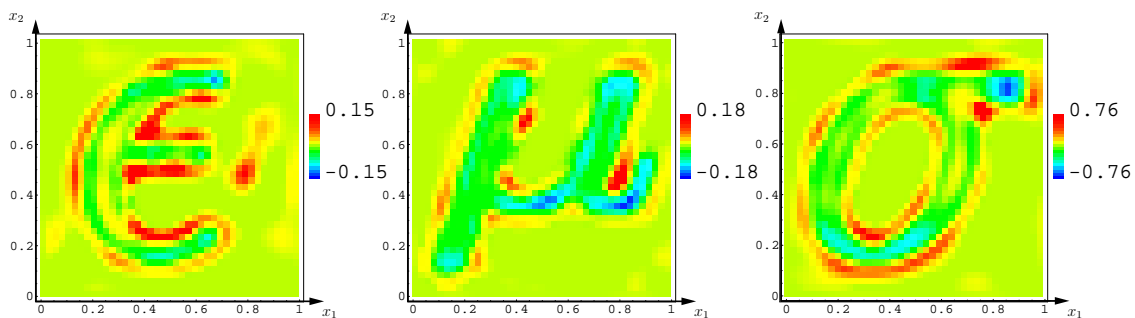
Figure 8.10: Error in the identified material parameters. From left to right: the permittivity, the permeability, and the conductivity, respectively.
