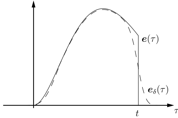
Figure 2.1: Smoothed function in the proof of F→T.
