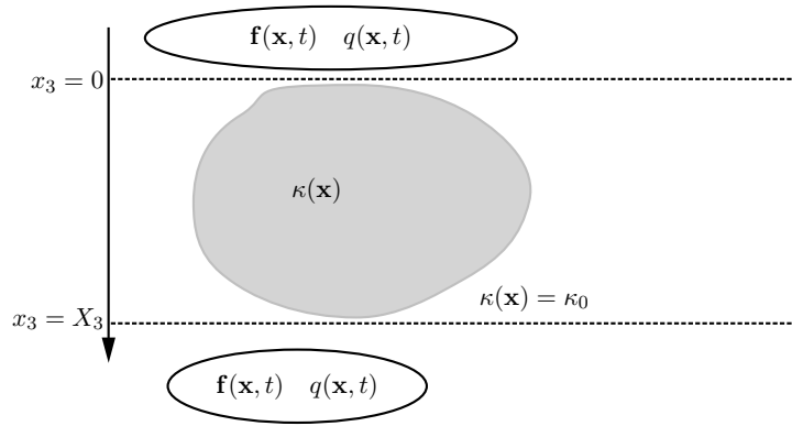
Figure 4.6: The acoustic scattering geometry.
