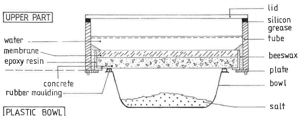
Fig. 3. The measuring method.
