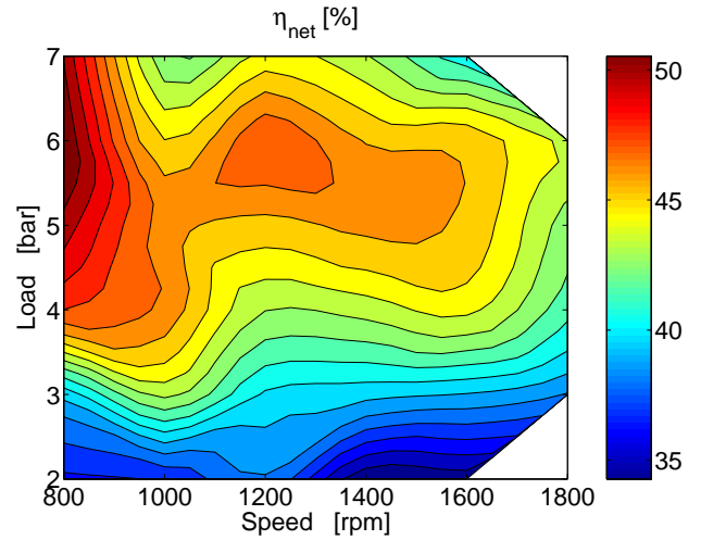
Figure 13: Net indicated efficiency. Engine run according to boost strategy.
