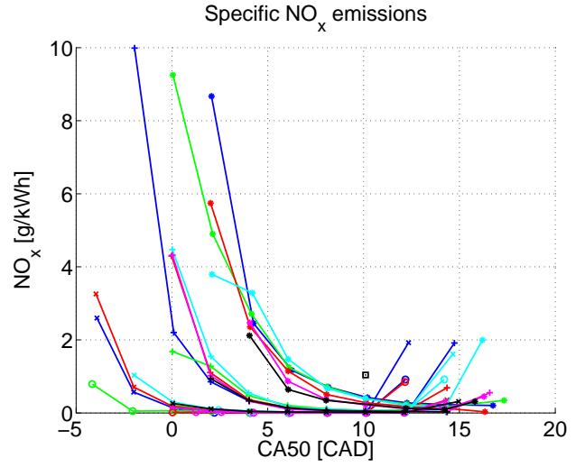
Figure 3: NO_x emissions as a function of combustion phasing (MIP operation). Legend can be found in Table 3.
