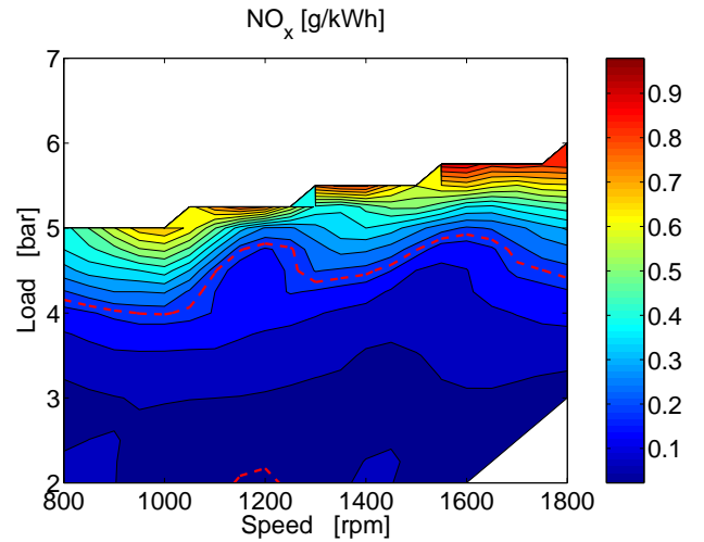
Figure 4: NO_x emissions (MIP operation). Red dashed line indicate limit of 0.2 g/kWh.
