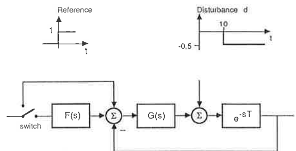
Fig. 7. Control system configuration for the integrator with time delay.
