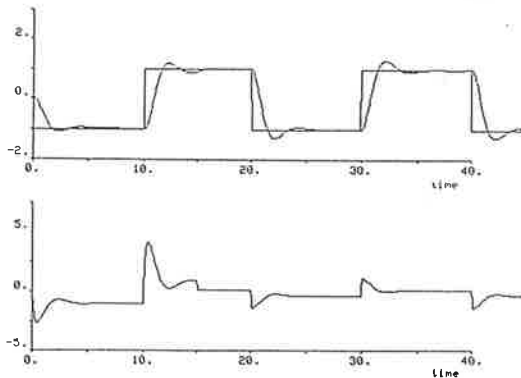
Fig. 3 Simulation of the robust control system. The gain is changed from 1 to 4 at time t=15s . The time constant is 1.
