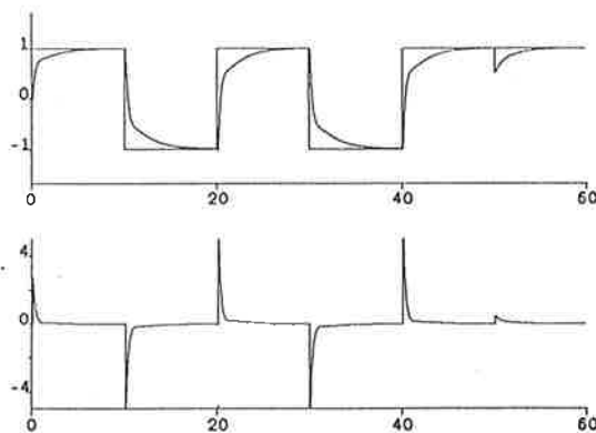
Fig. 9. Step response and step disturbance rejection for control with the robust regulator when T_d = 0.1 .
