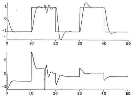
Fig. 5 Simulation of the adaptive control system. The gain is changed from 1 to 4 at time t=15s . The time constant is 1.
