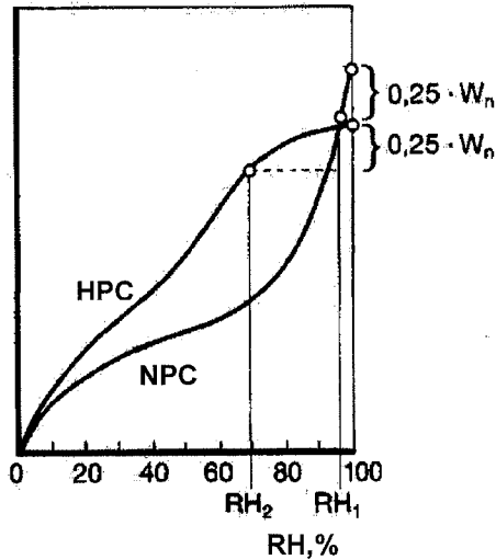
Figure 2.5 Sorption isotherm of HPC compared to NPC (Fagerlund, 1994)
