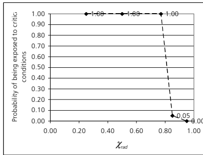
Figure G138. The individual risk to the most exposed person in the building, P_{worst}
