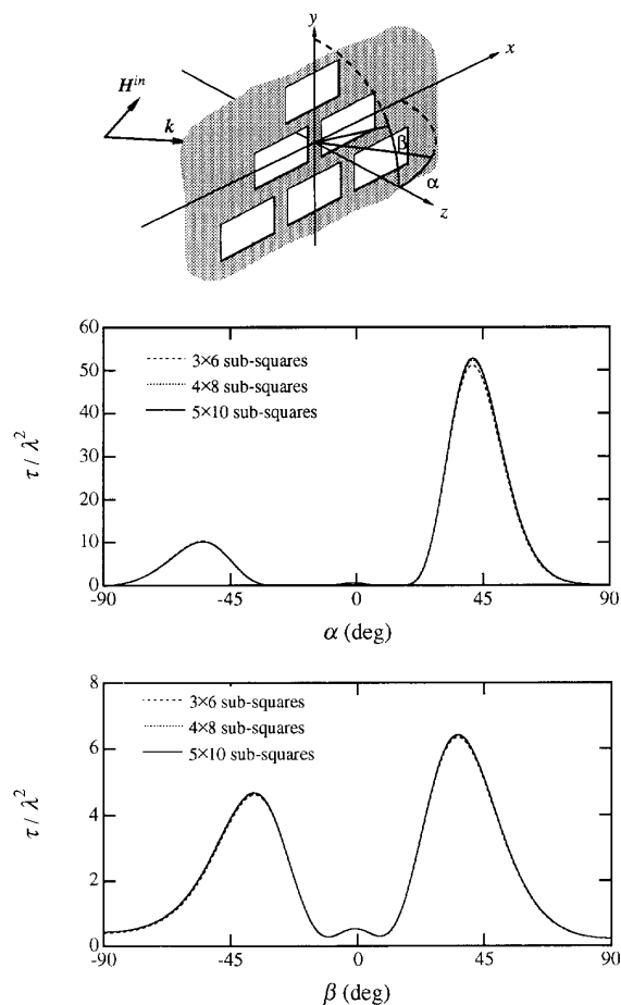
Fig. 14. Transmission cross section of a configuration of six apertures. The size of each aperture is 0.5\lambda \times 1\lambda and the distances between the apertures are 0.25\lambda . The results of three different discretizations of the apertures are illustrated. The plane of incidence is equal to the x - z plane and the incident angle is 45^\circ . The polarization of the magnetic field is perpendicular to the y axis.
