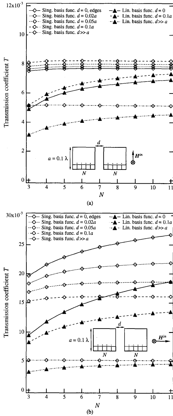
Fig. 5. Convergence of the transmission coefficient T for two square apertures, each with length of side a = 0.1\lambda . Normal incidence. Each aperture is divided into N \times N "subsquares." The convergence is shown for different distances d between the apertures. The polarization of the incident magnetic field is (a) transverse; (b) parallel to the row of apertures.
