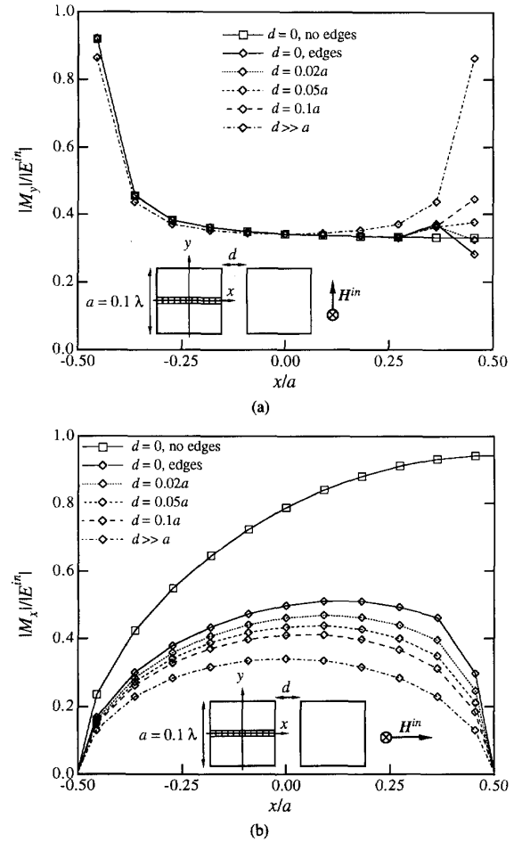
Fig. 6. The dominant component of the magnetic current density in one of two adjacent square apertures. Normal incidence. The mean values of the current density on "subsquares" in the middle row parallel to the row of apertures are shown. The length of the side of each aperture is 0.1\lambda . The apertures are divided into 11 \times 11 "subsquares." The polarization of the incident magnetic field is (a) transverse; (b) parallel to the row of apertures.
