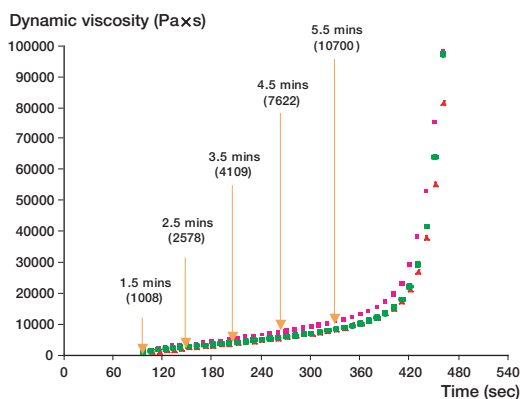
Figure 4. Viscosity profile of Palacos R bone cement.
