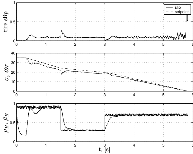
Figure 2.20 Simulation results for left back-wheel with HPID controller. Controlled braking is initiated on a high friction surface, then surfaces with lower friction are encountered. The tire slip has to be controlled at a given set-point value.
