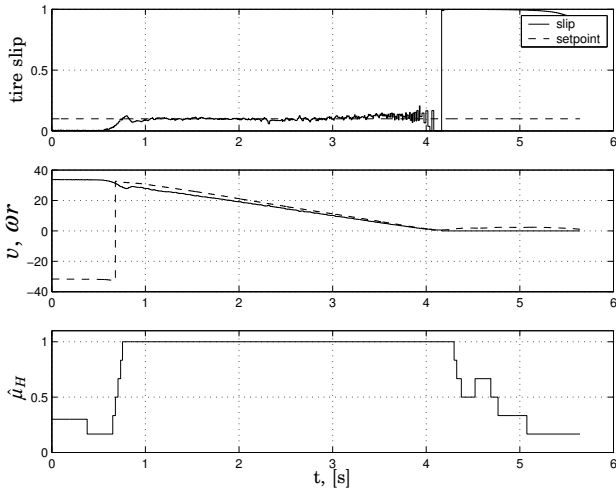
Figure 2.23 Experimental results for left back-wheel with HPI controller. Controlled braking is performed on dry asphalt. The tire slip has to be controlled at a given set-point value.
