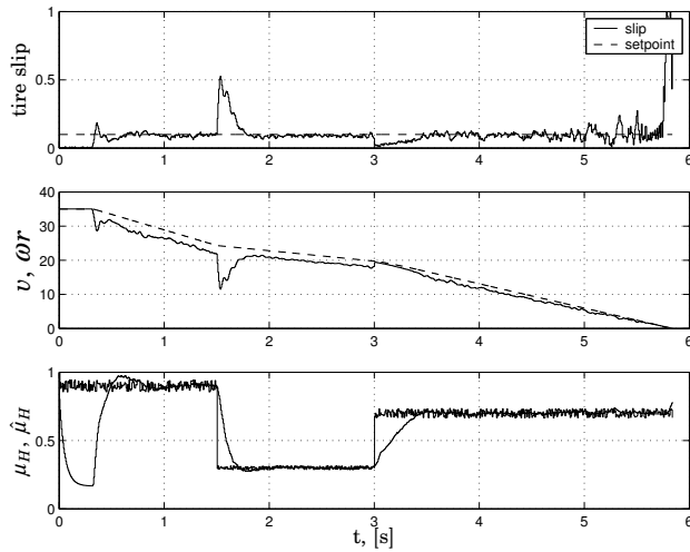
Figure 2.17 Simulation results for right front-wheel with HPID controller. Controlled braking is initiated on a high friction surface, then surfaces with lower friction are encountered. The tire slip has to be controlled at a given set-point value.
