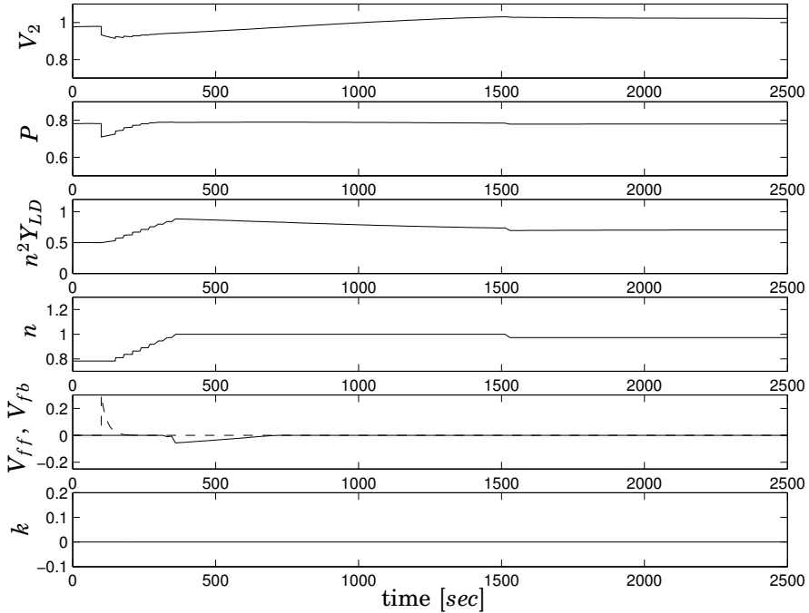
Figure 5.21 At t = 100 seconds, a line tripping is simulated by a 20% increase of the line impedance Z_{LN} . By momentary changes of the reference value by augmentation with V_{ff} (dashed line) and V_{fb} , stability is maintained without shedding load. In case the reference voltage had been kept constant, the system would become unstable.
