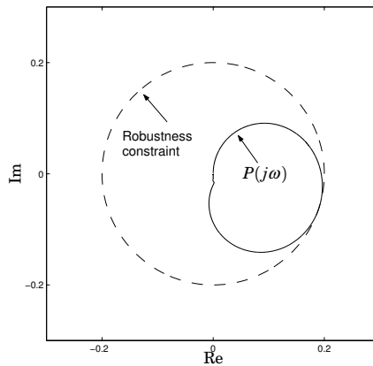
Figure 3.8 Nyquist plot of P(s) in Example 3.2.
