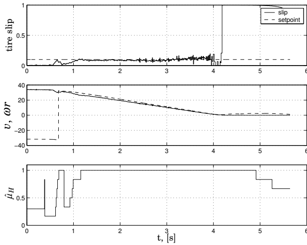
Figure 2.21 Experimental results for right front-wheel with HPI controller. Controlled braking is performed on dry asphalt. The tire slip has to be controlled at a given set-point value.
