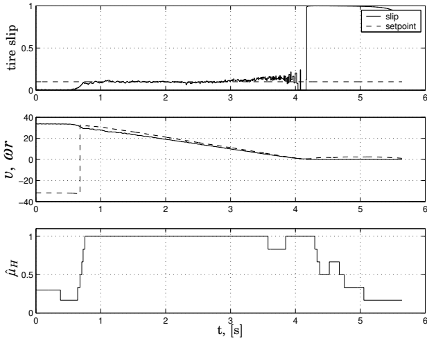
Figure 2.22 Experimental results for right back-wheel with HPI controller. Controlled braking is performed on dry asphalt. The tire slip has to be controlled at a given set-point value.
