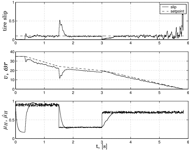
Figure 2.18 Simulation results for left front-wheel with HPID controller. Controlled braking is initiated on a high friction surface, then surfaces with lower friction are encountered. The tire slip has to be controlled at a given set-point value.
