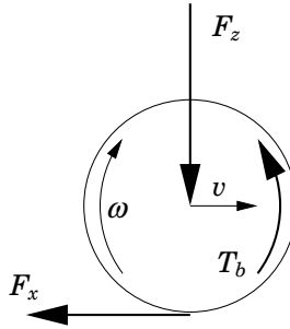
Figure 2.1 The quarter car consists of a single wheel attached to a mass.
