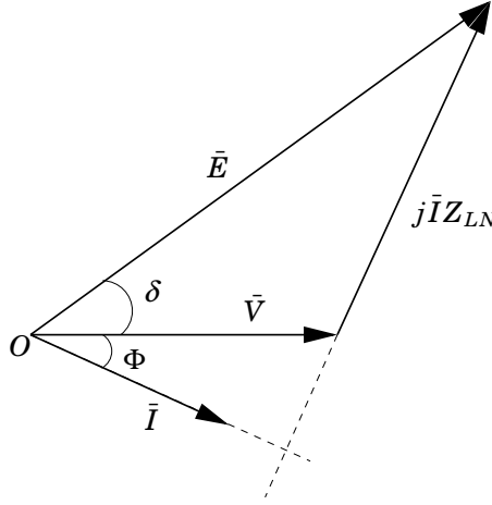
Figure 5.2 Phasor diagram for the considered power system.
