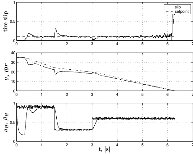
Figure 2.16 Simulation results for right back-wheel with HPI controller. Controlled braking is initiated on a high friction surface, then surfaces with lower friction are encountered. The tire slip has to be controlled at a given set-point value.
