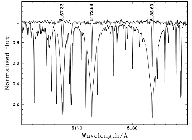
Fig. 6. Spectrum of the Sun and the metal-deficient star CD –24°17504 in the region of the Mg I b lines. The signal-to-noise ratio in the latter star is approximately 100, giving noticeable noise in the continuum, whereas the solar spectrum is almost noise-free. The 5167 Å member of the triplet is blended with an iron line in both stars, but the two longer wavelength transitions are free of significant blends in the metal-deficient star.
