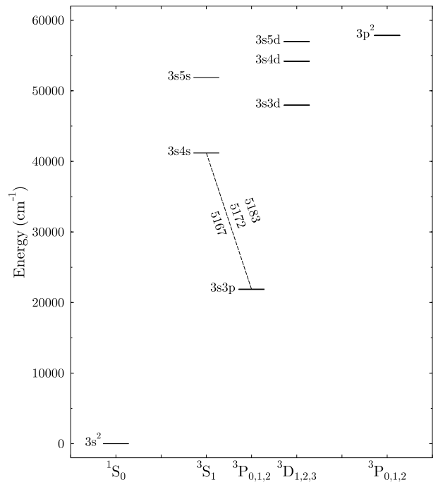
Fig. 1. Partial energy level diagram of Mg I displaying the ground state, the 3s3p\ ^3P levels and the levels for which the lifetimes have been measured in this work. The 3p – 4s lines are marked with wavelengths in Å.
