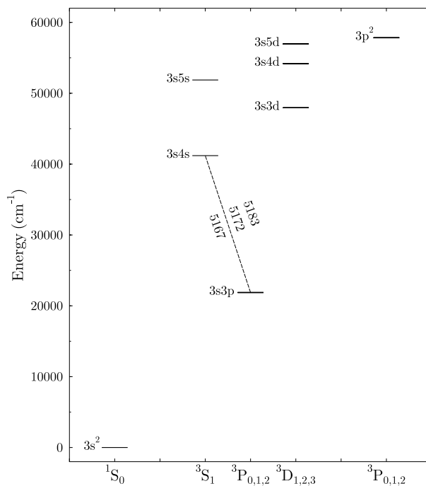
Fig. 1. Partial energy level diagram of Mg I displaying the ground state, the 3s3p\ ^3P levels and the levels for which the lifetimes have been measured in this work. The 3p-4s lines are marked with wavelengths in Å.
