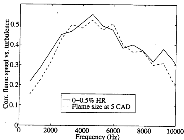
Figure 9 Correlation of flame speed versus turbulence as a function of turbulence frequency.
