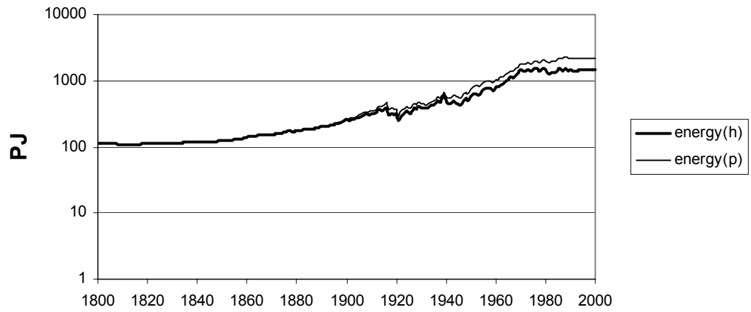
Figure 6: Aggregate energy consumption in Sweden 1800-2000, in PJ, lin-log scale.
