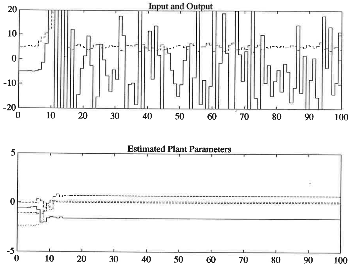
Figure 2. Input and output measurements as well as parameter estimates for system of Table 2.
