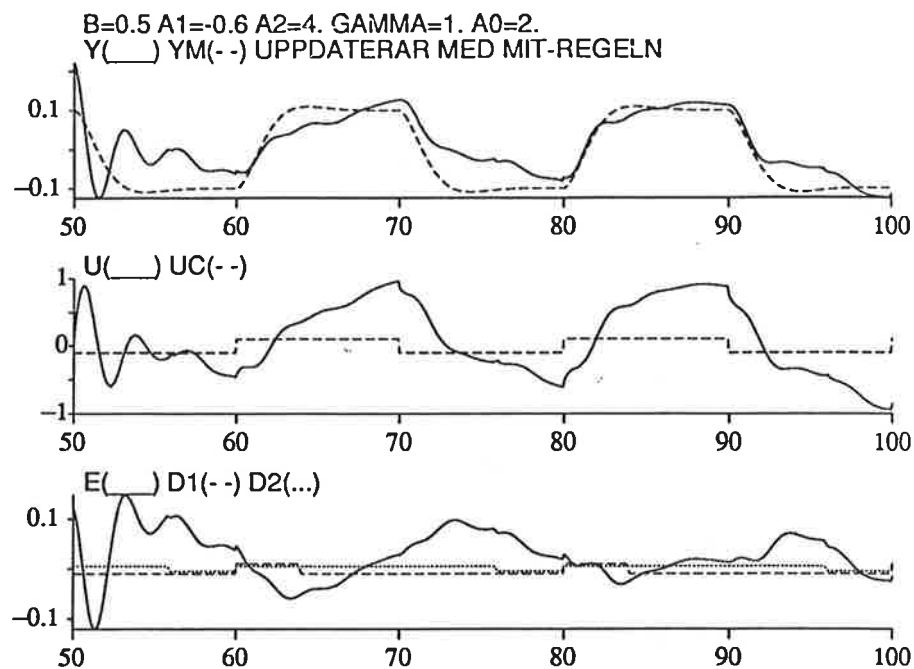
Figur 3.6 MIT-regulator polerna i HHP
