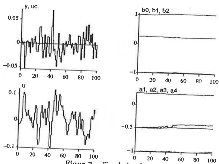
Figure 2. Simulering 2
