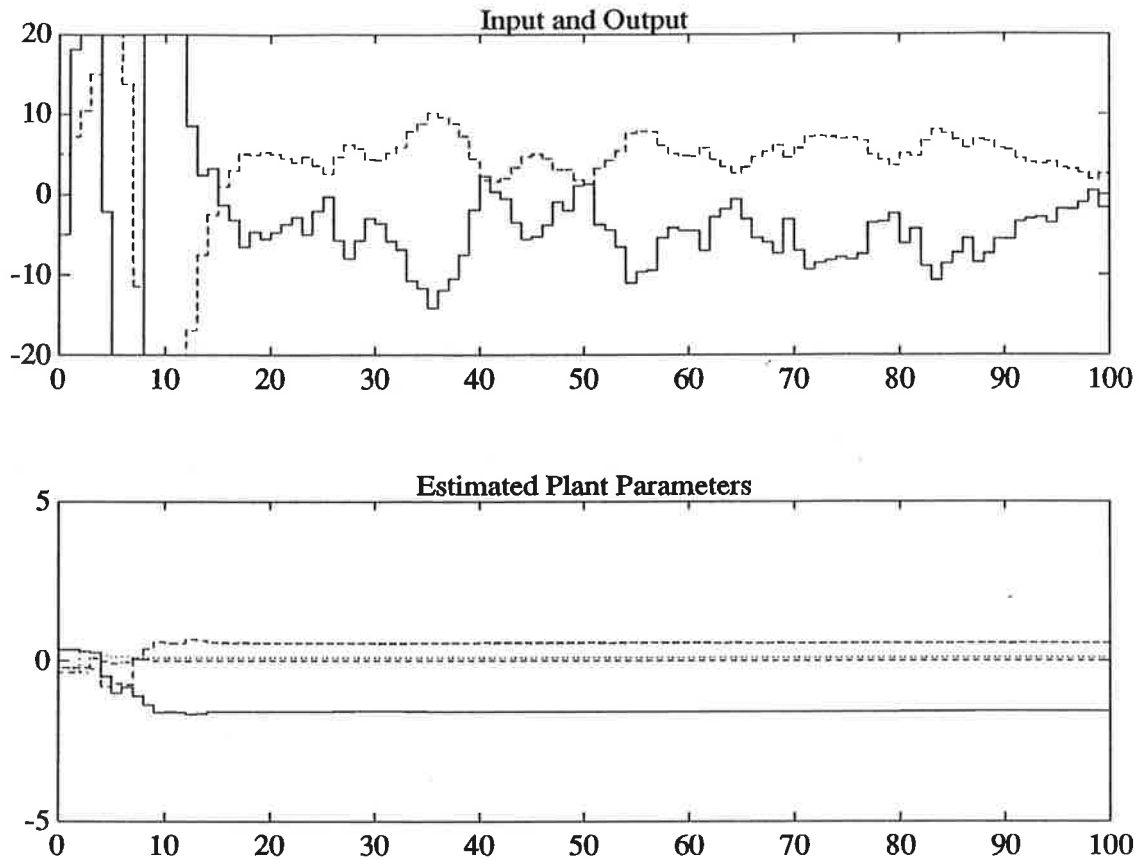
Figure 1. Input and output measurements as well as parameter estimates for the second order system using a pole placement regulator. Note that to separate the plots of y and u these have been displaced by 5 and -5 units respectively.
