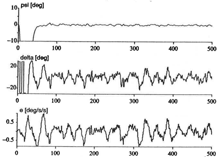
Figure 4.2 Minesweeper, with feedforward
