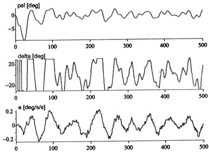
Figure 4.3 Cargo ship, without feedforward
