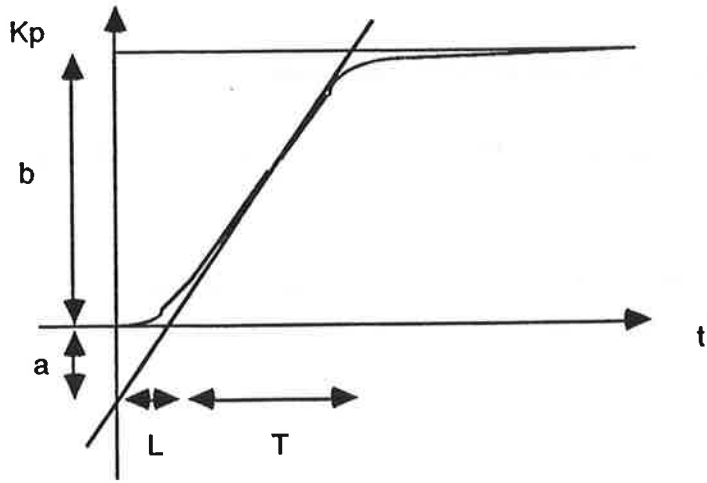
figure 2.1 Step response
