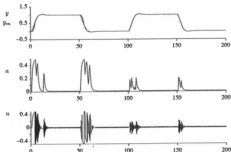
Figur 4. K = 1 ; 0 < t < 100 , K = 25 ; 100 < t < 200
