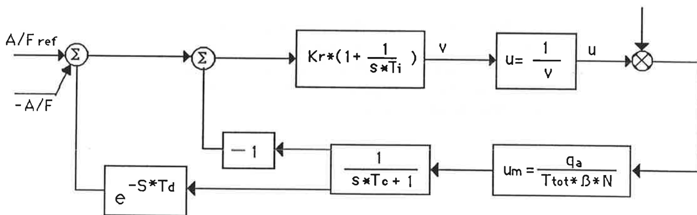
Figur 6 Regulator
