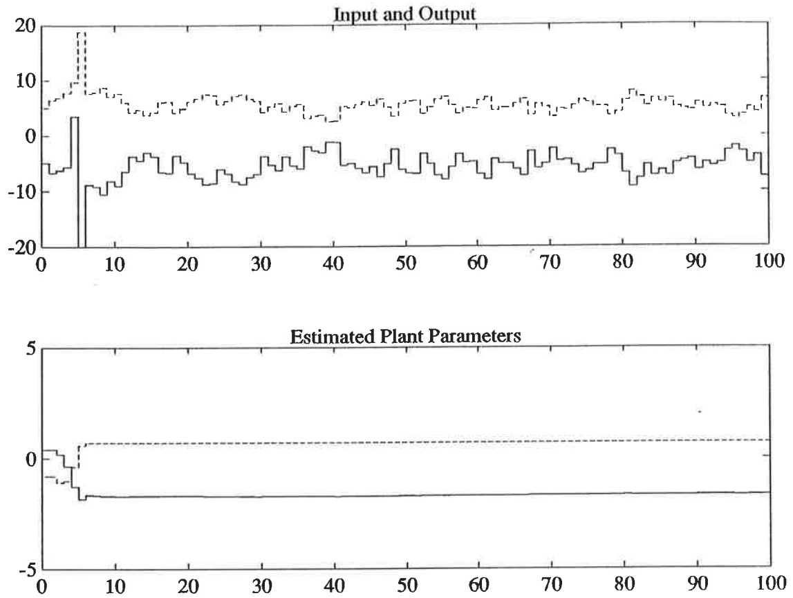
Figure 3. Input and output measurements as well as parameter estimates for system of Table 3.
