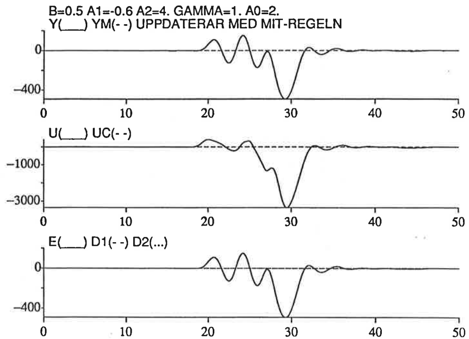
Figur 3.5 MIT-regulator polerna i HHP
