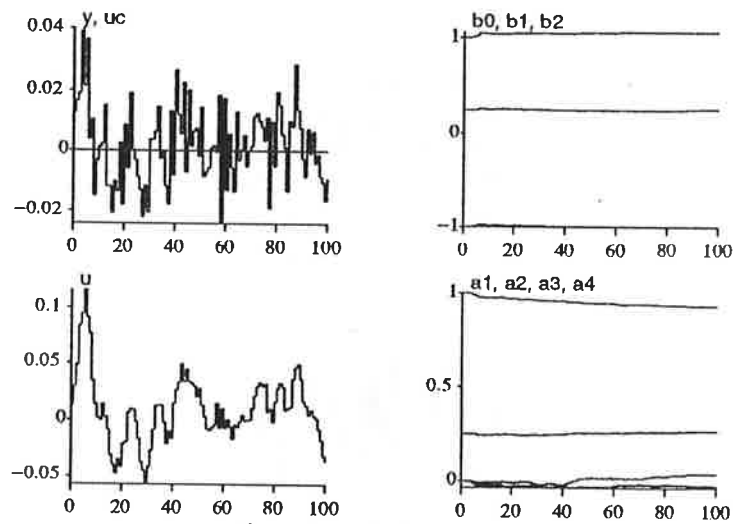
Figure 6. Simulering 6
