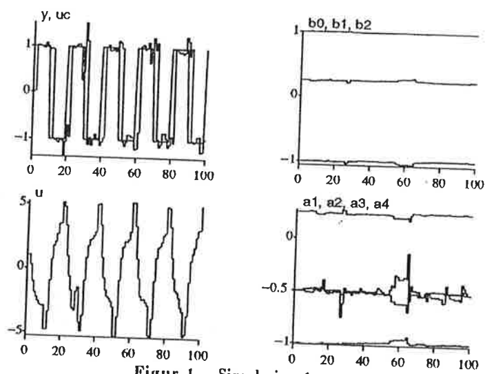
Figure 1. Simulering 1
