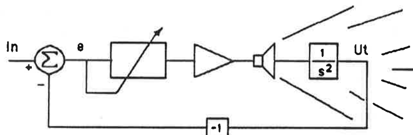
Figur 3.1 Blockschema
