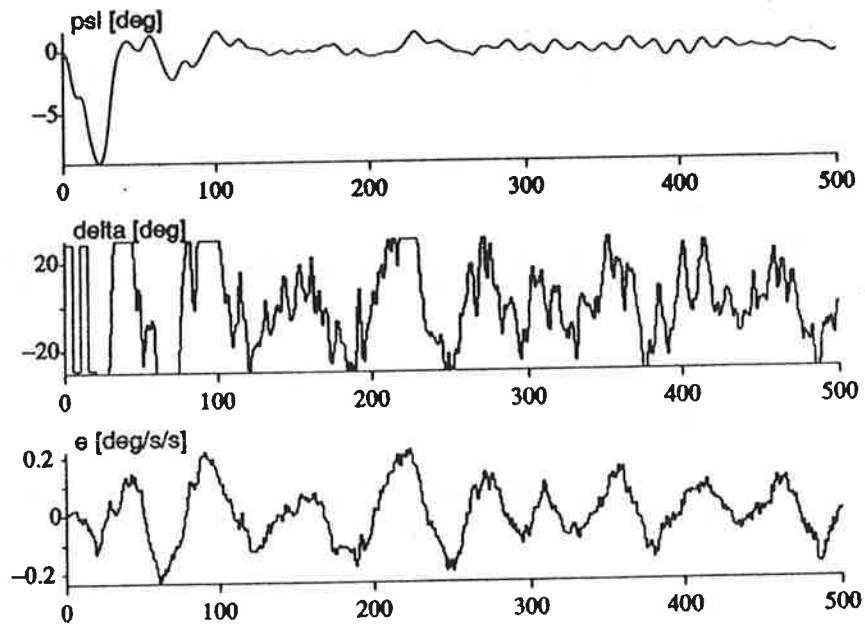
Figure 4.4 Cargo ship, with feedforward
