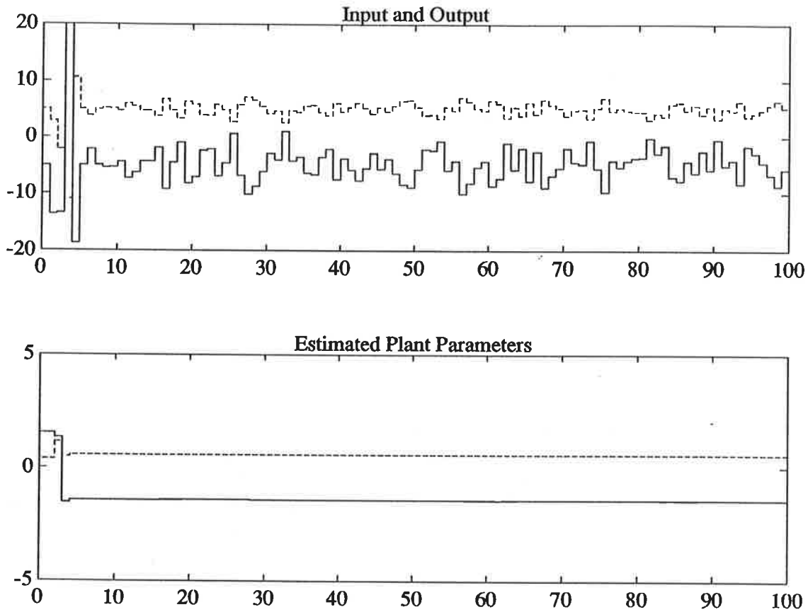
Figure 4. Input and output measurements as well as parameter estimates for system of Table 4.
