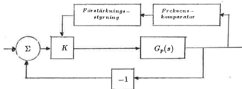
Figur 9. General Electrics system.
