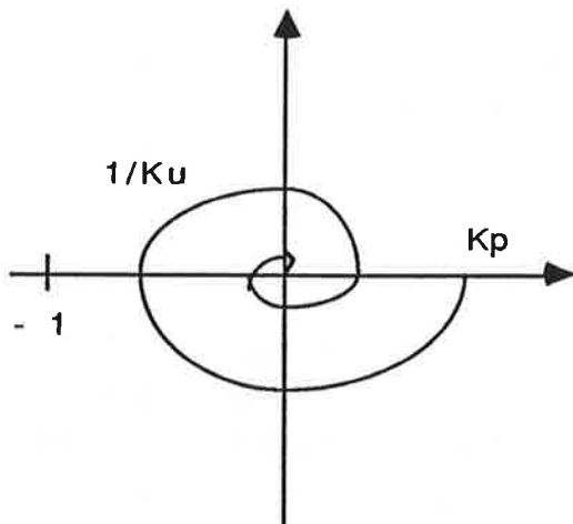
figure 2.2 Nyquist curve for frequency response.
