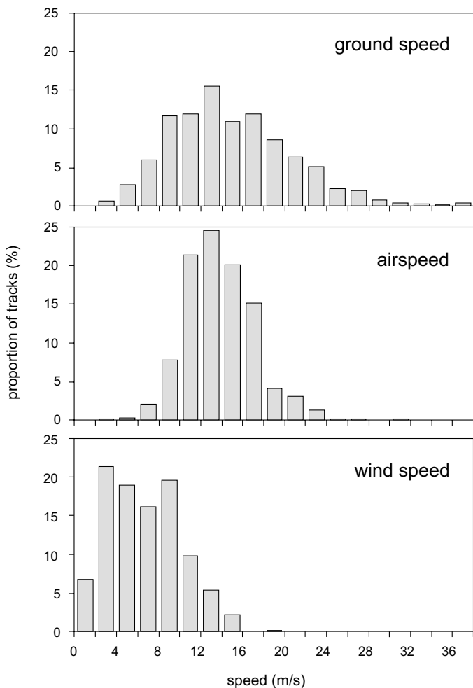
FIG. 6. Distribution of ground speed ( n = 692 ), air speed ( n = 644 ), and wind speed ( n = 644 ) for the total sample of radar tracks.
