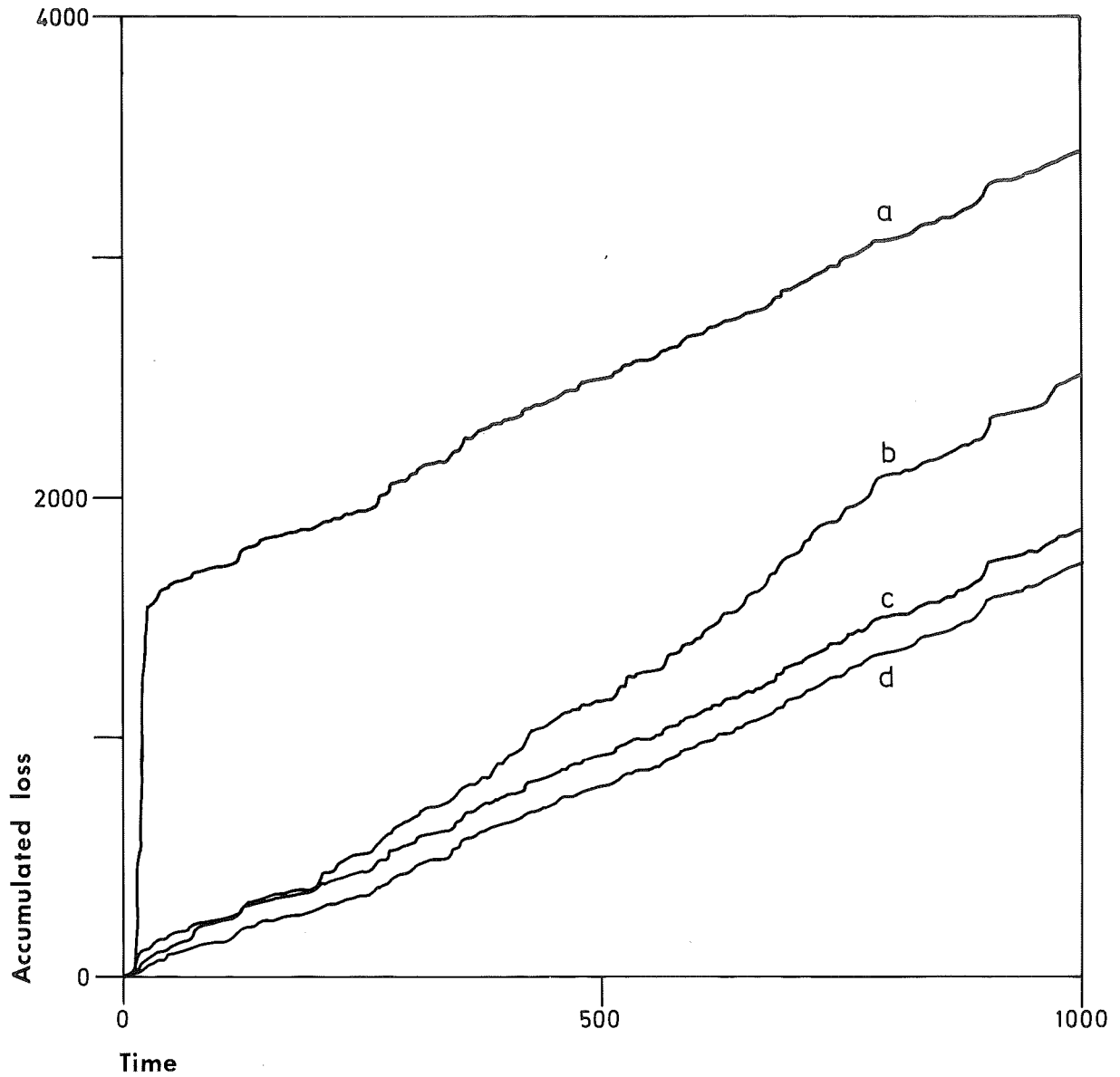
Fig. 3.3 - Accumulated loss, \sum y(t)^2 , for different regulators and limitations of the input signal. a. Self-tuning regulator no limitation b. - " - - " - |u| \leq 1 c. - " - - " - |u| \leq 5 d. Controller (3.3) |u| \leq 5
