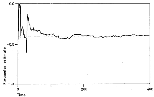
FIG. 3. Parameter estimate a(t) obtained when the self tuning algorithm based on the model (7.3) is applied to the system given by (7.1). The minimum variance regulator corresponds to a = -0.4 and is indicated by the dashed line.
