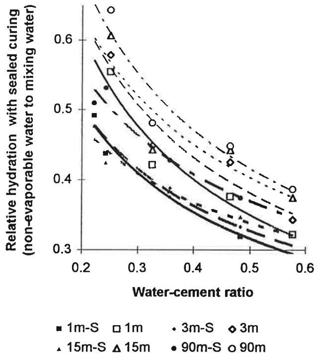
Fig. 19 - Relative hydration (non-evaporable water to mixing water) in concrete with sealed curing. m= months; S= 10% silica fume
