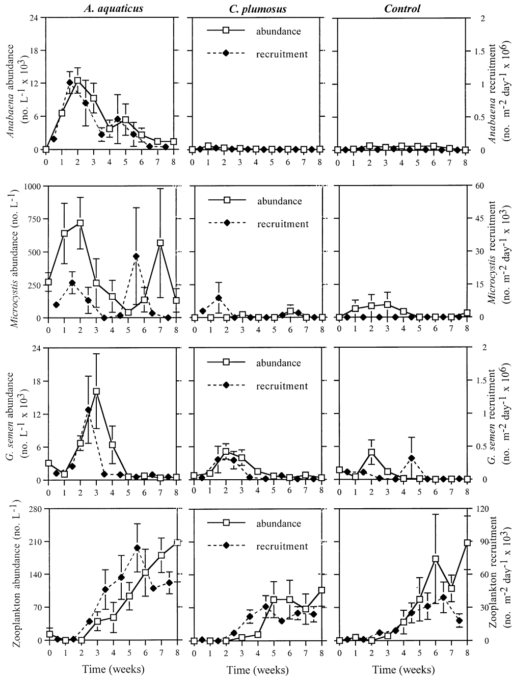
Fig. 1. Abundance (individuals L -1 ) and recruitment (individuals m -2 d -1 ) of Anabaena , Microcystis , G. semen , and major zooplankton groups (cladocerans, copepods, and Asplanchna ) during 8 weeks of sampling, including one pretreatment sampling (week 0), in different treatments ( Asellus aquaticus , Chironomus plumosus , and Control). Note that the scales are different for different organisms.
