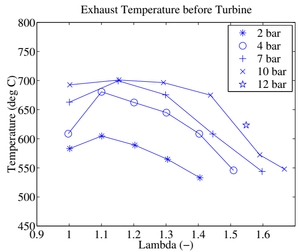
Figure 10. Exhaust temperature before turbine, at lean operation with ignition set to minimize NOx emissions, for various load cases.
