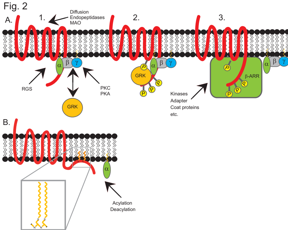
Fig. 2 – Schematic representation of covalent modifications and protein-protein interactions involved in receptor desensitization. A, steps (1-3) in receptor desensitization. B, receptor-efector acylation. RGS - regulator of G protein signaling; \beta -ARR - beta-arrestin.
