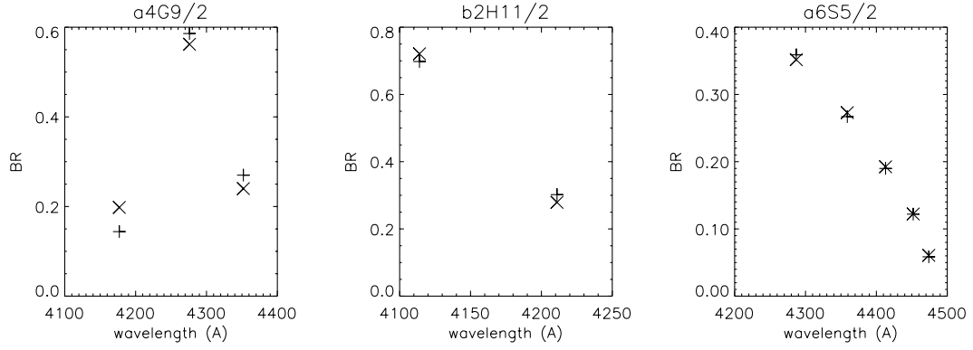
Fig. 3. Branching ratios for the metastable levels a^4G_{9/2} , b^2H_{11/2} and a^6S_{5/2} . Crosses (×) mark the astrophysical values corrected for reddening and the (+) mark the theoretical values (Quinet et al. 1996).
