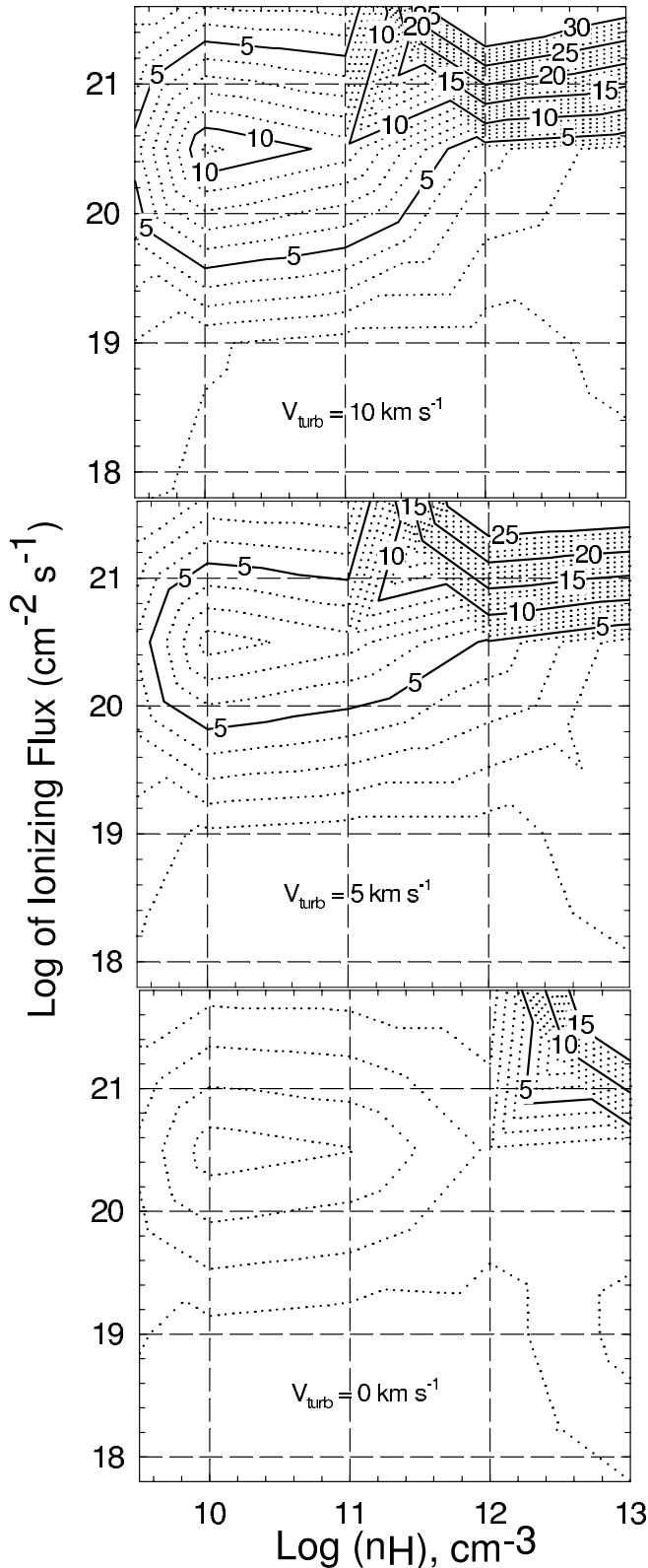
FIG. 2.— \text{Fe II (UV)}/\text{Mg II} ratios predicted using the 830 level model for \text{Fe}^+ in a QSO BLR as a function of the hydrogen density n_{\text{H}} and the flux of hydrogen-ionizing photons. The chemical abundances are solar, the cloud column density is 10^{24} \text{ cm}^{-3} , and v_{\text{turb}} = 0, 5, \text{ and } 10 \text{ km s}^{-1} .
