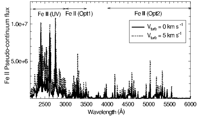
FIG. 1.—Fe II pseudo-continuum predicted by the 830 level Fe + model for physical conditions in QSO BLRs, n_{\text{H}} = 10^{12} cm -3 , \log \Phi_{\text{ion}} = 20.5 cm -2 s -1 . The 2200–6000 Å wavelength range is divided into small bins of 6 Å (consistent with a \sim 500 km s -1 FWHM at 3600 Å) and the Fe II flux is calculated in each bin. The model at v_{\text{turb}} = 0 km s -1 predicts many strong and narrow Fe II features in the 1600–3500 Å range (solid line). The same model, but at v_{\text{turb}} = 5 km s -1 , is marked by dashed lines.
