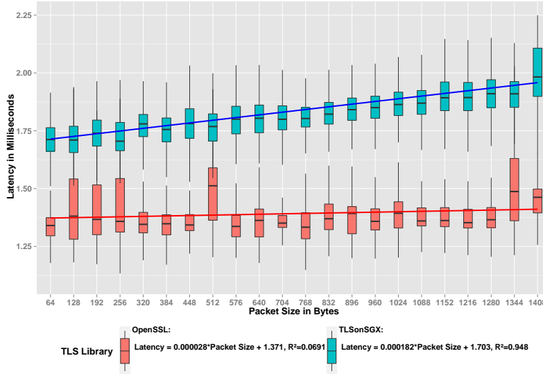
Fig. 5. UDP Packet Round Trip Latency vs. Packet Size
