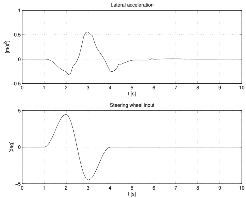
Figure 62 Lateral acceleration and steering input.
