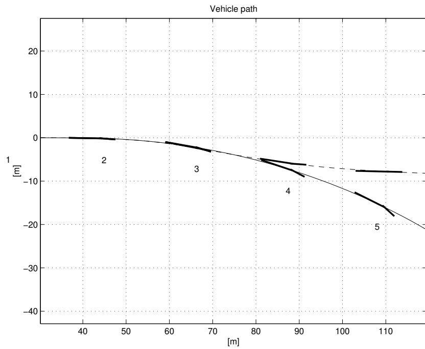
Figure 65 Vehicle trace for the linear reference model (dashed), and the controlled model with nonlinear tires.
