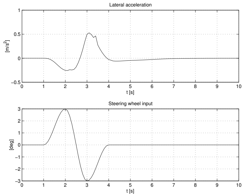
Figure 72 Lateral acceleration and steering input.
