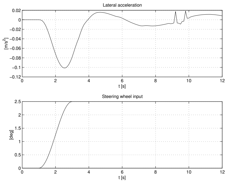
Figure 47 Lateral acceleration and steering input.
