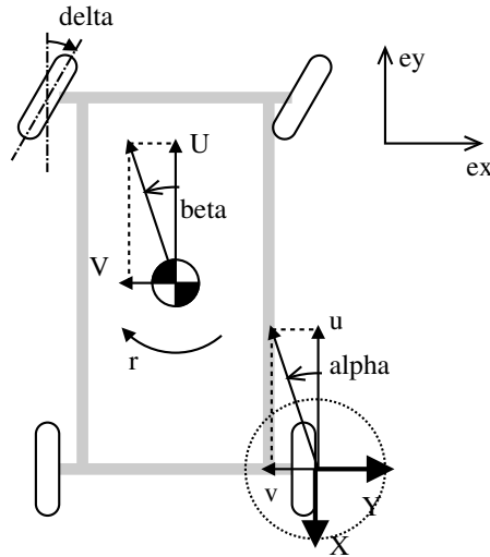
Figure 1 Illustration of velocities and forces on the car.
