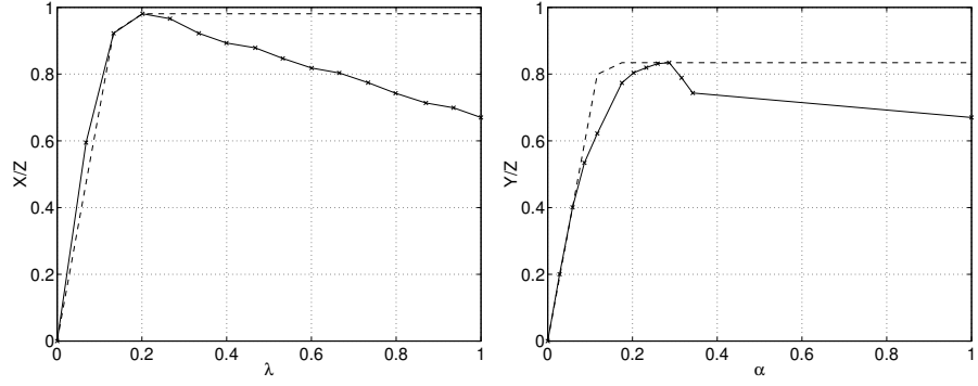
Figure 7 Saturated linear adhesion forces (dashed) compared to experimental data (solid). The experimental data is obtained from Volvo Truck Corporation [Edl91].
