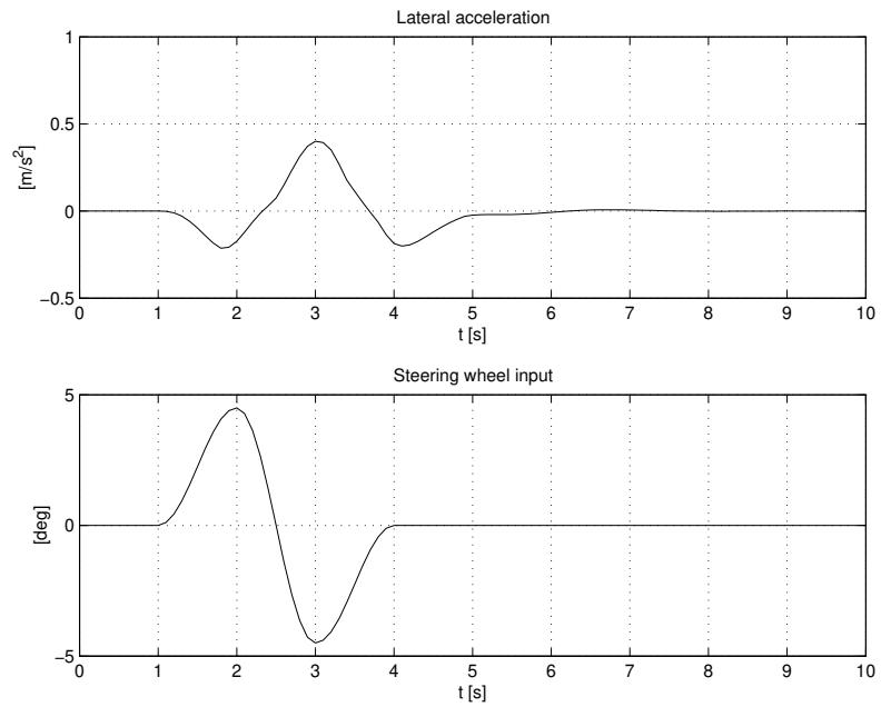
Figure 52 Lateral acceleration and steering input.
