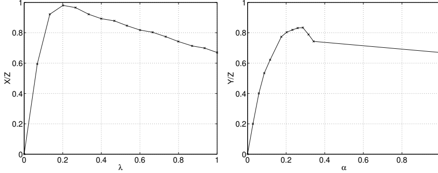
Figure 6 Experimental tire adhesion coefficients at pure braking and pure cornering. The last data value for the lateral adhesion coefficient is estimated as being equal to the longitudinal adhesion coefficient for \lambda = 1 . The experimental data is obtained from Volvo Truck Corporation [Edl91].
