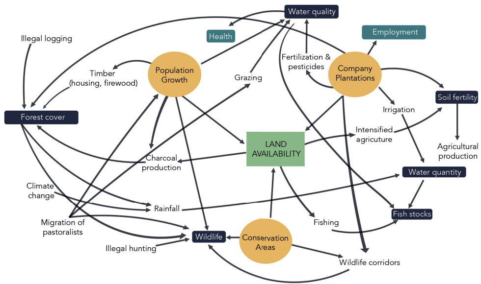
Figure 13. Causal loop diagram that represents the main drivers, impacts, and feedbacks of socio-environmental change in Kilombero Valley.
