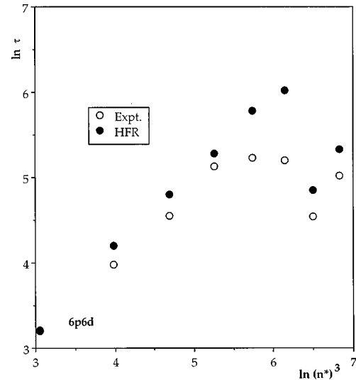
FIG. 5. Same as Fig. 4 but for the 6pnd 1/2[5/2]_2^o levels.
