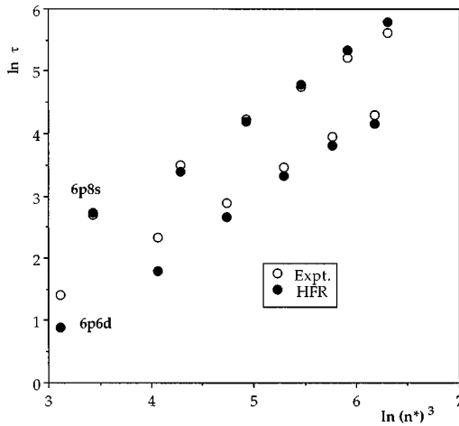
FIG. 4. Comparison of the experimental (○) and theoretical (●) lifetimes for the 6pns (1/2, 1/2)_1^o (upper curves) and 6pnd 1/2[3/2]_1^o (lower curves) states. \log_e \tau is plotted vs \log_e [(n^*)^3] . The straight line indicates proportionality with respect to (n^*)^3 .
