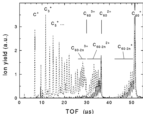
FIG. 1. Typical TOF spectra after ionization and fragmentation of C_{60}^+ with near-infrared femtosecond laser pulses. All data shown in this Letter were obtained below the apparent ionization threshold of Xe, i.e., in an estimated intensity range \approx 10^{13} - 10^{14} W/cm 2 . Solid line: medium intensity in this range; dashed line: maximum intensity
