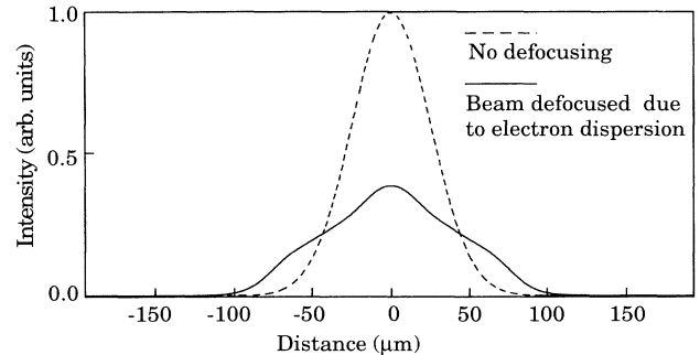
FIG. 6. Intensity at the focus as a function of transverse distance from the optical axis, illustrating ionization-induced defocusing of the fundamental laser beam in the alkali-metal plasma. The peak intensity for this modeling, in the absence of defocusing, was chosen to be 10 times the saturation intensity of the neutral atoms remaining in the plasma.
