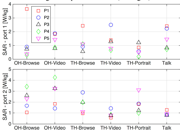
Fig. 6. Peak SAR in 6 user scenarios at 859 MHz.
