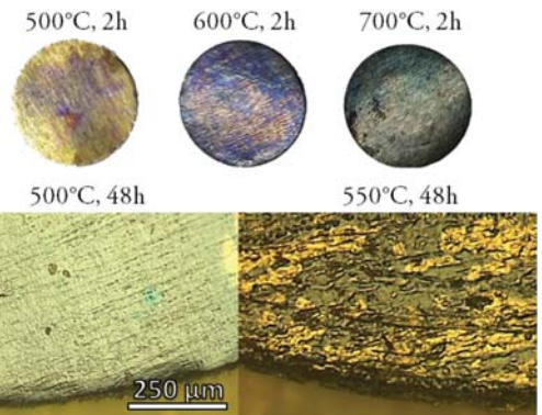
Fig. 5. Surface images of tungsten foils (5.5 mm dia.) after oxidation in argon containing maximum 5 ppm of oxygen.
