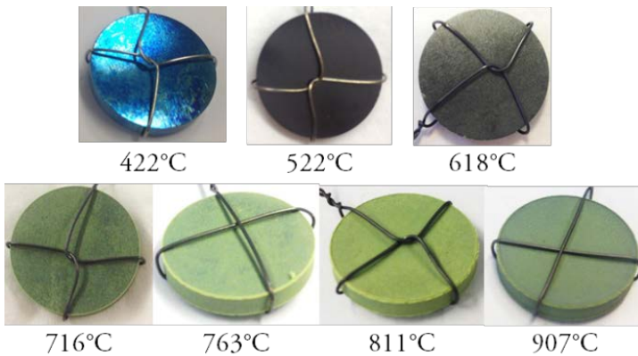
Figure 29 Specimens after oxidation for 2h in a He-0.5% \text{O}_2 gas mixture.
