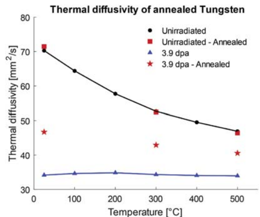
Fig. 2. Thermal diffusivity of annealed tungsten at 25–500 ^\circ\text{C} .
