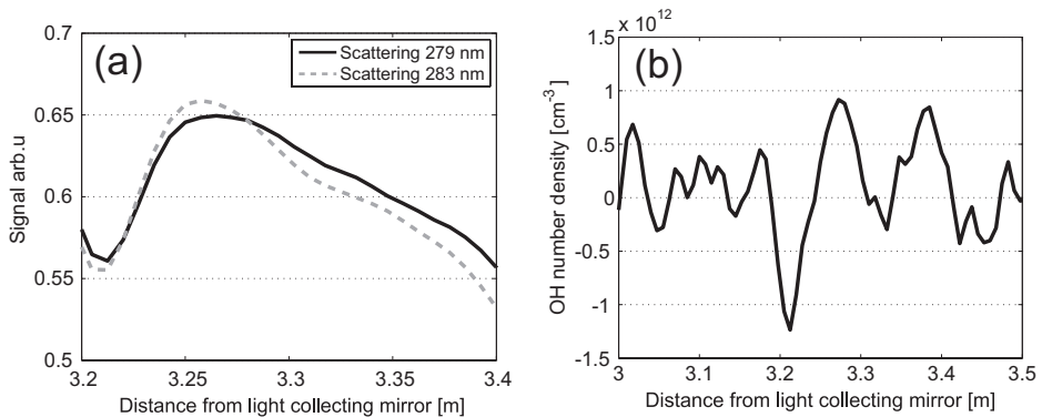
Figure 6.10 Measurement of OH with a slot burner positioned at \sim 3.2 m. Panel (a) shows the lidar signals from the on- and off resonance wavelengths, 283 and 279 nm, respectively. In (b) the evaluated concentration profiles are shown. The most prominent feature, the negative peak, is probably due to resonance fluorescence giving a positive signal contribution to the lidar curve at the on resonance wavelength 283 nm, which is seen as the overshoot at 3.25 m in (a).
