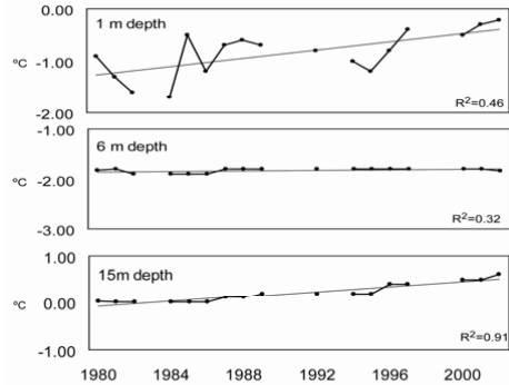
Figure 4. Ground temperatures at 1, 6 and 15 meters depth and linear trends at Kursflaket mire measured in September from 1980 to 2002.
