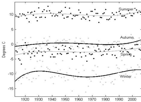
Figure 2. Seasonal air temperatures and a 4 th degree polynomial fit from the Abisko Scientific Research Station, 1913-2006.
