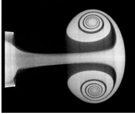
Figure 1.10 – Fluid entrainment during vortex formation, here shown for L/D = 2.0 104 visualized using planar laser-induced fluorescence (PLIF). After formation, the vortex ring consists of both ejected fluid from inside the cylinder (grey) and ambient fluid (black) pulled into the vortex ring from the vicinity of the nozzle.
