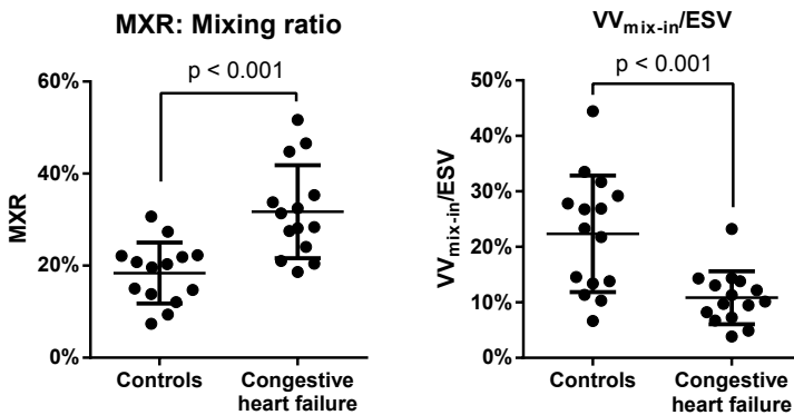
Figure 5.14 – Comparison of mixing ratio (MXR) and VV mix-in /ESV, the fraction of the end-systolic volume mixed into the vortex ring during early rapid filling, between healthy volunteers and patients with congestive heart failure. (Paper V)
