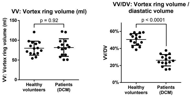
Figure 5.13 – Vortex ring volume (VV, left) and VV in relation to the diastolic volume (DV), VV/DV (right), from Papers IV and V. For VV, no difference was found between patients and volunteers. However, a large difference was found in VV/DV. (Papers IV and V)
