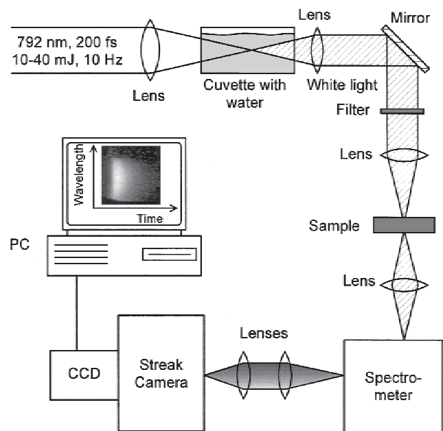
Fig. 2. Setup for time-resolved photon propagation studies using white light (from Andersson-Engels et al. , 1993).
