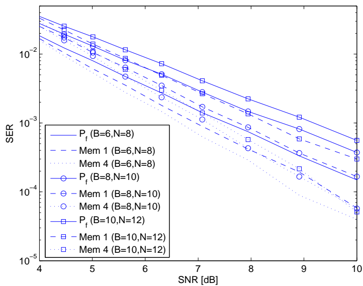
Figure 3.3: SER comparisons when B = N - 2 . Solid lines show the performance of P_f , which is the competing scheme from [65]. The dashed lines stand for the performance of the precoders that give a memory-1 structure on \mathbf{G} , while the dotted ones show the performance of the precoders that give a memory-4 cyclic structure on \mathbf{G} .
