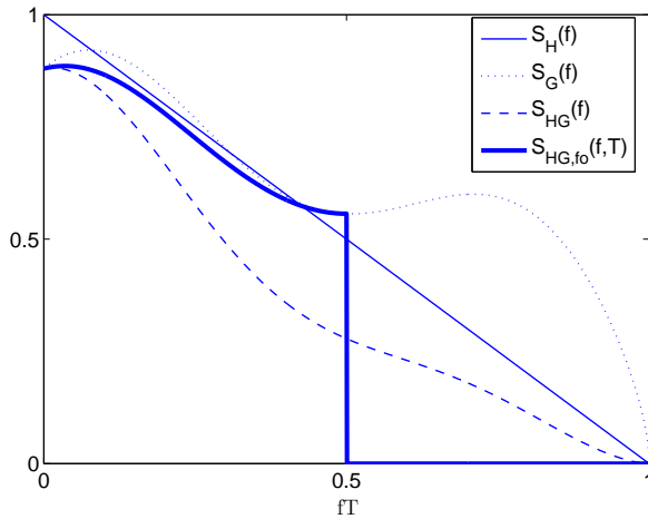
Figure 1.2: The quantities S_H(f) , S_G(f) , S_{HG}(f) and S_{HG,f_0}(f, T) . Note how folding occurs around the point f = 1/2T .
