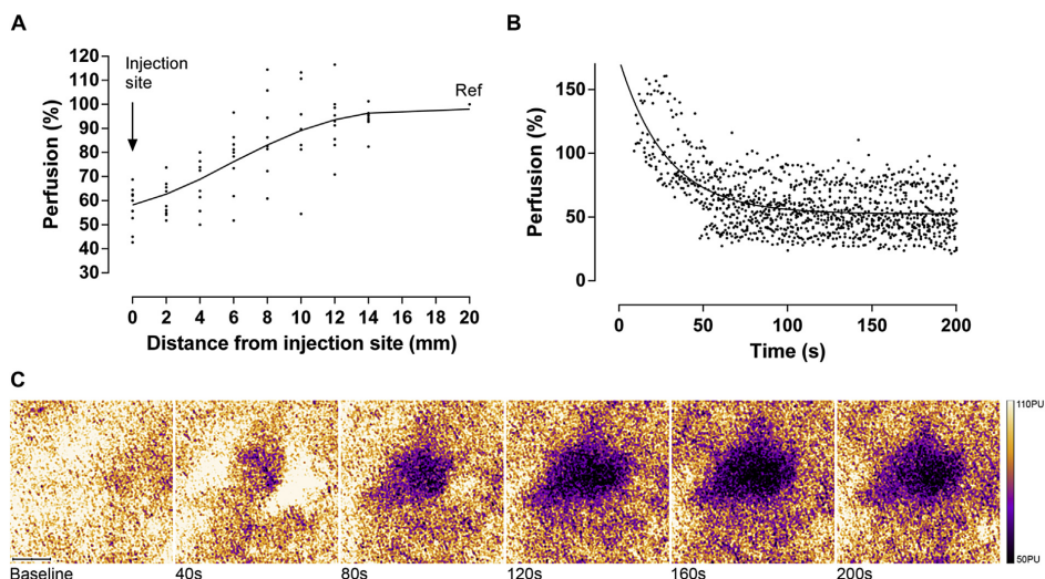
Figure 4 Blood perfusion after a single injection of lidocaine + epinephrine (20 mg/ml lidocaine + 12.5 \mu g/ml epinephrine). Panel A shows the distance the hyperperfusion spread from the injection site in intact skin ( n = 9 ). Perfusion was measured every 2 mm from the injection site 120 s after injection using LSCI. The results are expressed as percent of a reference point (Ref) 20 mm from the injection site. Note that the hyperperfusion spread to a radius of 12 mm from the injection site. Panel B shows the drop in perfusion over time ( n = 7 ). Perfusion was measured in flaps using LSCI. Perfusion is expressed as percent of the baseline value before the experiments were started (defined as 100%) and analysed using non-linear regression analysis (one-phase decay), reaching a maximum after 121 s (95% confidence interval of 107–136 s). The experiments went on for 5 min. The graph illustrates what happens in the first 200 s, and beyond this time-point, there was no further change. Panel C is a representative example of an experiment that shows the spread of the hypoperfusion over time and area. Saline was injected after baseline recordings as a negative control, and the results showed no change in perfusion. Perfusion was measured by LSCI of intact skin on the pig flank, and the results are expressed in the arbitrary units, perfusion units (PU). The scale bar (bottom left) is 10 mm.
