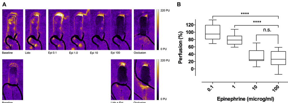
Figure 3 Blood perfusion in flaps after the injection of increasing concentrations of epinephrine. Panel A is a representative example of an experiment in which blood perfusion was measured using LSCI. Baseline measurements were performed before the experiments were started. Saline was injected after baseline recordings as a negative control, and the results showed no change in perfusion. The upper row shows the injection of lidocaine (Lido) followed by increasing concentrations of epinephrine (Epi 0.1, 1.0, 10 or 100 \mu\text{g}/\text{ml} ). The lower row shows the injection of lidocaine + epinephrine (20 mg/ml lidocaine + 12.5 \mu\text{g}/\text{ml} epinephrine). The experiments were concluded by mechanically occluding the base of the flap using a ligature (occlusion). Perfusion is expressed in the arbitrary units, perfusion units (PU), as defined by the scale. Panel B is a box plot showing the results from the injection of increasing concentrations of epinephrine where perfusion was measured using LDV and LSCI ( n = 9 ). The box denotes the 25–75th percentiles, the whiskers denote the minimum and maximum values (range) and the line denotes the median. Perfusion is expressed as percent of baseline values. Maximal response was reached at a concentration of 10 \mu\text{g}/\text{ml} epinephrine. Statistical analysis was performed using Mann–Whitney U test; p < 0.0001 (****) and p > 0.05 (not significant, n.s.).
