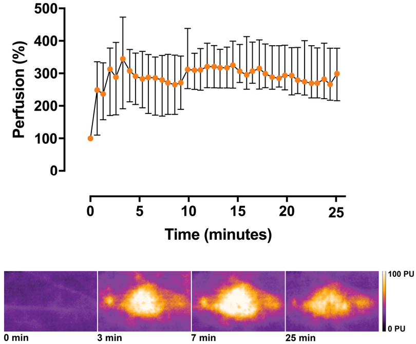
Figure 4. Results of LSCI, showing perfusion after the injection of 20 mg/ml lidocaine +12.5 µg/ml epinephrine. Representative images are shown before injection and 3, 7, and 25 min after injection. Note the paradoxical increase in signal intensity despite the fact that epinephrine is known to induce vasoconstriction and subsequent hypoperfusion. Data are presented as median values and interquartile ranges (% of baseline values). (From Paper V.)
