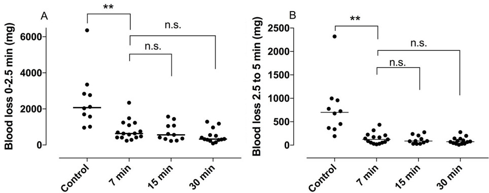
Figure 5. The amount of blood lost after the injection of lidocaine only (control), and after the injection of lidocaine + epinephrine (12.5 µg/ml), and waiting 7, 15, or 30 minutes before incision. (A) Bleeding during the first 2.5 minutes after incision (one point for control at 6257 mg is included in the calculations, but not shown in the graph), and (B) during the second 2.5 minutes after incision (one point for control at 2320 mg is included in the calculations, but not shown in the graph). (From Paper IV.)
