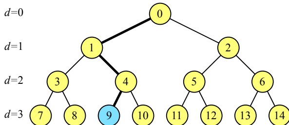
Figure 2: An example of a complete binary tree with the depths, d , of each level shown to the left. The node number is shown inside each node circle. For the blue node at the bottom, we have levelStart = 2^d = 2^3 and levelIndex = 2 , which makes it possible to compute the node number as 2^3 + 2 - 1 = 9 . For the blue node, we also have swapMask = 010 (in binary), which indicates the path from the root down to the node, where 0 is a descension in to the left child, and 1 is in to the right child. The swapMask is used in Algorithm 3.
