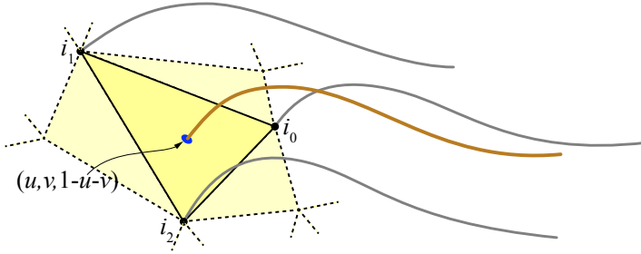
Figure 12: Part of a triangular control mesh is shown where the grey curves are thin control curves defined at the vertices of a darker yellow triangle. Given the thin control curves, a new thin curve (brown) can be represented by thin control curve indices, (i_0, i_1, i_2) , and barycentric coordinates, (u, v, 1-u-v) within that triangle. This is an extremely compact representation which is valuable when rendering large numbers of thin curves.
