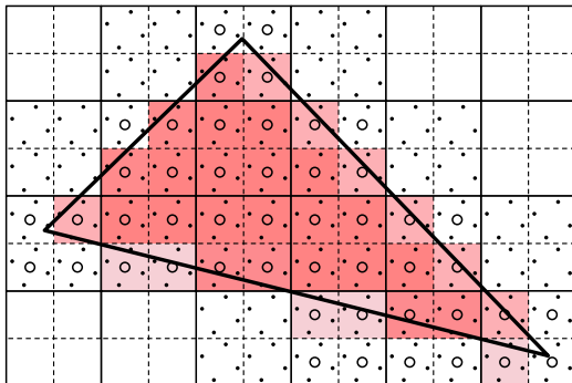
Figure 7: A triangle rasterized using 4 visibility and one shading sample per pixel ( 4\times MSAA). Four inside and depth tests are here performed per pixel, and the covered samples are used to blend shading between the background and the triangle. While not completely eliminated, aliasing along the triangle edges have noticeably improved compared to Figure 6.
