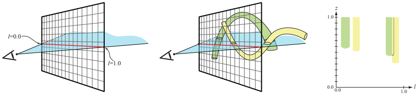
Figure 2: Left: a line sample is defined by the camera location and a line (red) in screen space, and parameterized by l . Middle: two curves with thickness intersect the line sample. Right: visibility is resolved in the l - z -plane by finding the closest surfaces in depth, z , along l . As can be seen, the yellow thin curve occludes part of the green thin curve over this line sample to the right, but not to the left.
