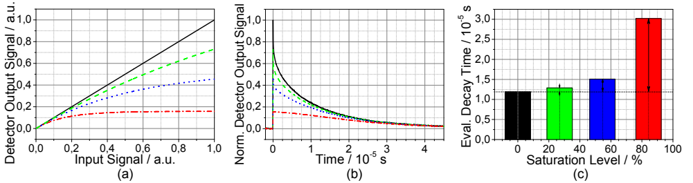
Figure 4.31: Example of how different saturation states in the detector (a) change the shape of the output time-signal (b) and the evaluated decay time (c). The original decay transient in (b) (—) corresponds to an average of 100 measured signal curves of La_2O_2S:Eu at room temperature.
