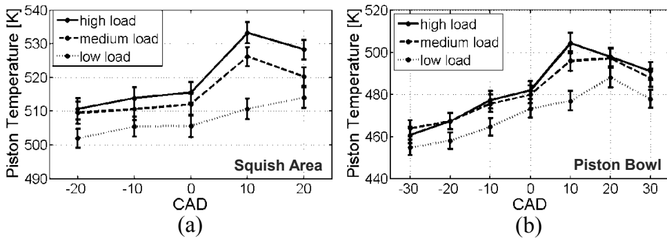
Figure 5.2: Piston surface temperature transients of an optical heavy-duty research engine during HCCI combustion around TDC. Temperatures measured for three different loads, obtained in the squish area (a) and in the piston bowl (b), are displayed. The temperature values and standard deviations (see error bars) correspond to measurements of 100 consecutive and averaged engine cycles.
