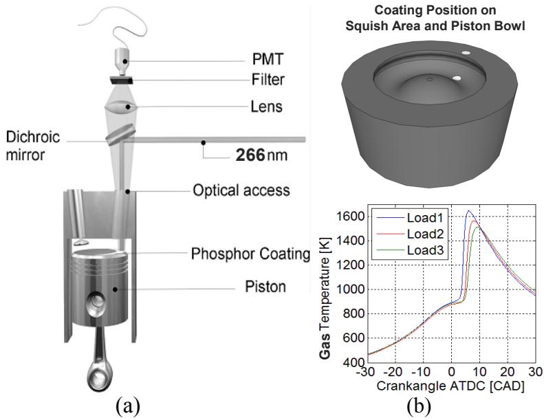
Figure 5.1: Part (a): The experimental setup employed for obtaining dual-point measurements of piston temperatures through use of LIP. Part (b): Three different engine loads were compared, as shown in terms of the global gas temperature transients, which were extracted from the pressure trace inside the cylinder.
