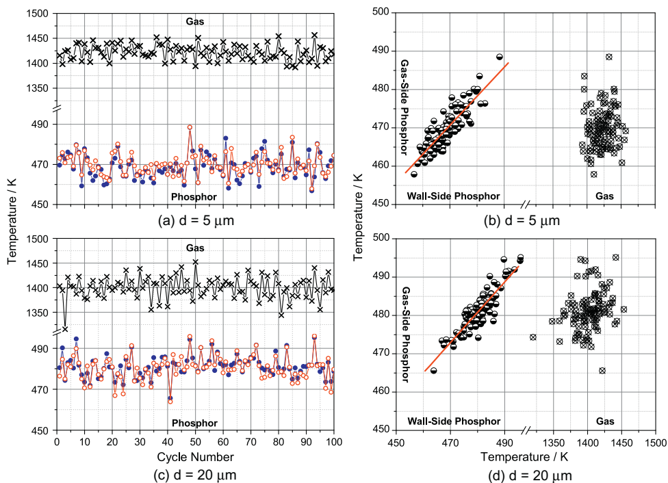
Fig. 10. Cycle-to-cycle variations of gas and phosphor temperatures, measured at 20 CAD ATDC during fired engine operation using \text{La}_2\text{O}_3\text{:S:Eu} coatings. The upper figure part, (a) and (b), originates from data taken with a 5\ \mu\text{m} coating whereas the lower part, (c) and (d), shows temperatures from a 20\ \mu\text{m} coating. Data indicators: cross = global gas temperature, circles/dots = phosphor temperature (red circle = gas-side, blue dot = wall-side), half-hollow circle = phosphor temperature correlation, cross + circle = gas vs. phosphor-gas-side temperature correlation.
