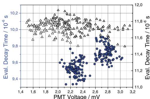
FIG. 9. Comparison of response slopes for two different phosphors (blue dots: \text{La}_2\text{O}_2\text{S:Eu} at 473 K; black triangles: \text{CdWO}_4 at 308 K) at similar decay times, using equal PMT gains (4700 and 6300) and laser energies that yield the same decay signal voltages.
