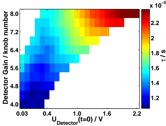
Figure 4.32: Detector response matrix of a PMT (Hamamatsu H6780-04), measuring \text{CdWO}_4 phosphorescence at 294 K. The evaluated decay time is shown as a function of the gain knob number and the detector peak voltage.
