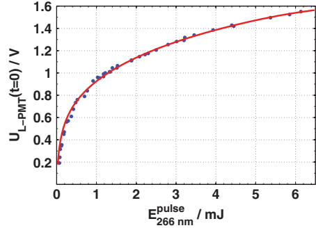
FIG. 2. Fitted correlation (red line) showing the signal peak voltage from L-PMT in as a function of Laser pulse energy. The gain of the L-PMT was set to a constant value of 6300 and additional transmission losses T_{L-PMT} were introduced (see Figure 1) in order to prevent detector damage.
