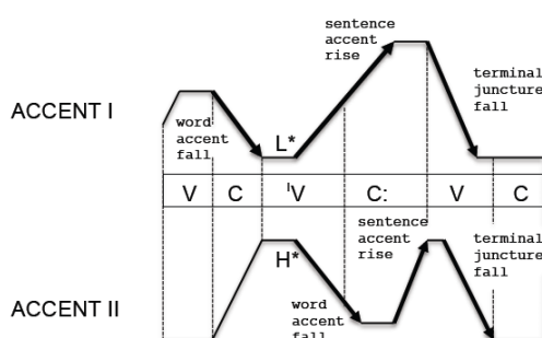
Figure 2. Timing difference of same basic tonal pattern in the realization of Accent 1 and Accent 2 in relation to the CV-tier. Note the low tone at the beginning of the stressed vowel ( l V) in Accent 1 and the high tone at the beginning of the stressed vowel in Accent 2 (adapted from Bruce 1977 and Bruce 1986).
