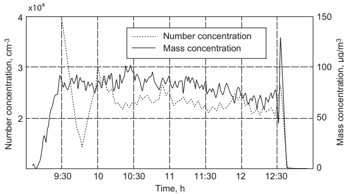
Fig. 7. The variation of terpene–ozone particle mass concentration and number concentration during a typical generation event. Ozone and aerosol generation starts at 9:00. The event starts at 09:30 and finishes at 12:30.
