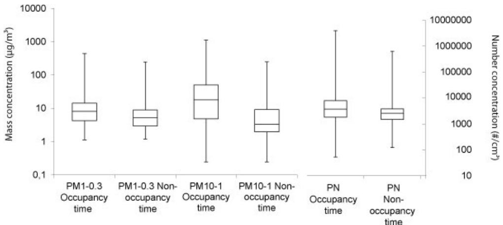
Figure 5. Boxplots of particle mass concentrations ( \text{PM}_{1-0.3} and \text{PM}_{10-1} ) (left) and particle < 300 nm number concentration (right) during occupancy and non-occupancy time. The boxes denote the quartiles, the horizontal line the medians and the whiskers maximum and minimum concentrations.
