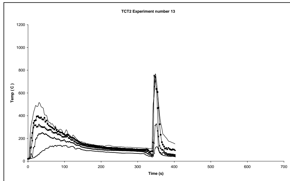
Figure A16. Temperature-time graph for experiment number 13.
