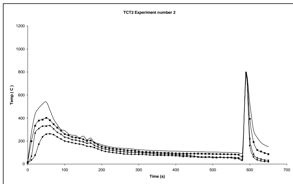
Figure A5. Temperature-time graph for experiment number 2.
