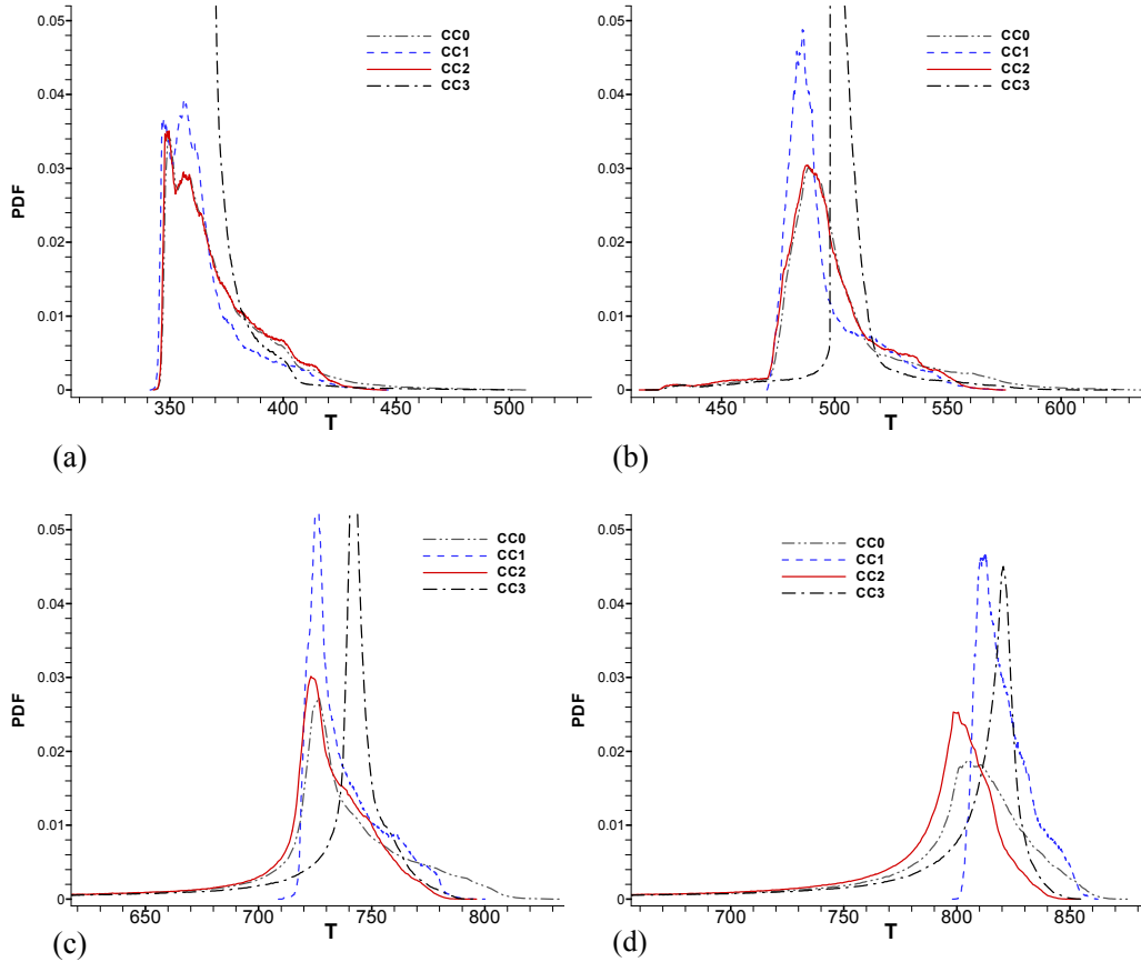
Figure 22: The temperature PDF during compression stroke. (a) CAD 240; (b) CAD 300; (c) CAD 330; (d) CAD 360.
