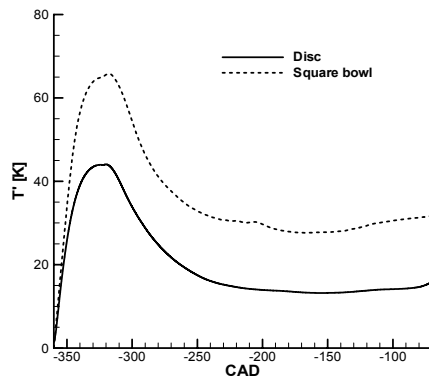
Figure 29: Evolution of temperature inhomogeneity in the two engines from LES. The computation starts from intake at -360CAD.
