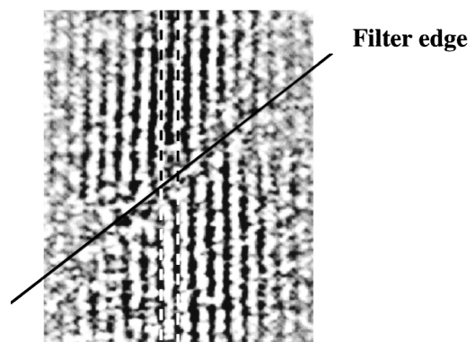
Fig. 2. Interference pattern with the 13th harmonic through an aluminum step filter (two-shot integration). The envelope of the spatial distribution of the harmonic beam is removed by use of a Fourier-transform technique.
