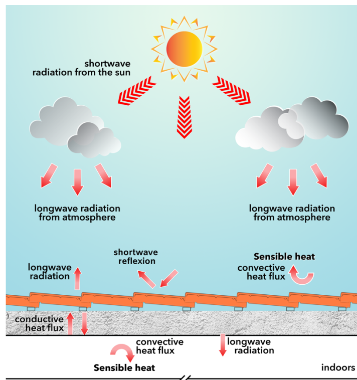
Figure 3.18: Energy balance of a conventional roof
