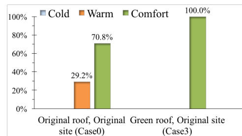
Figure 7.1: Percentage of hours below, within and above the comfort zone according to ASHRAE Standard 55, Original roof and Green roof, in the Original site, (Cases 0 and 3), Typical summer day
