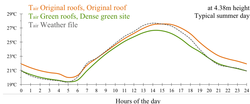
Figure 6.6: T_{air} for Original roofs in the Original site (Case 0) and Green roofs in the Dense green site (Case 5), at 0.13m above the plants, compared to T_{air} from the weather file, in the Typical summer day
