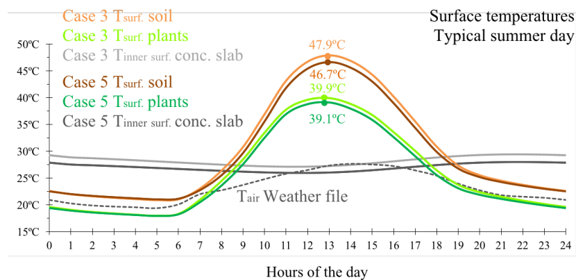
Figure 7.5: Surface temperatures of plants and soil, and inner surface of the concrete slab for the Green roof in the Original site (Case 3) and in the Dense green site (Case 5), compared to T_{air} from the weather file in the Typical summer day
