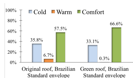
Figure 5.13: Percentage of hours below, within and above the comfort zone according to ASHRAE Standard 55, Original roof and green roof, Brazilian standard envelope, one-year period
