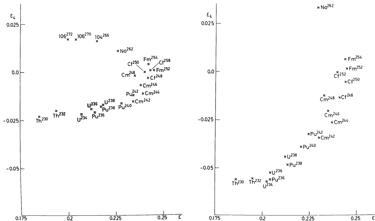
Fig. 1. Equilibrium \epsilon(Y_{20}) and \epsilon_4(Y_{40}) deformations in the actinide region with coupling between shells N_t and N_t \pm 2 neglected (left) and included (right).
