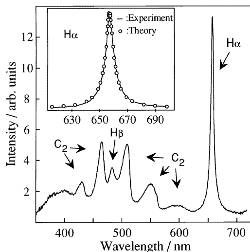
Figure 2. The spectrum from a breakdown arc. A theoretical Stark-broadened H_\alpha line profile is fitted to the spectrum yielding the electron density N_e = 8 \times 10^{17} \text{ cm}^{-3} . The voltage is 40 kV and the gap distance is 4 mm.
