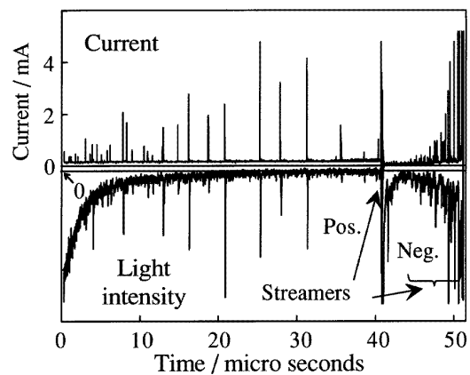
Figure 3. Current and (PMT) light recordings of laser-triggered electric breakdown. The electrode voltage is 43 kV, the gap distance is 4 mm and the laser pulse energy is 200 mJ. The baselines for both traces are marked.
