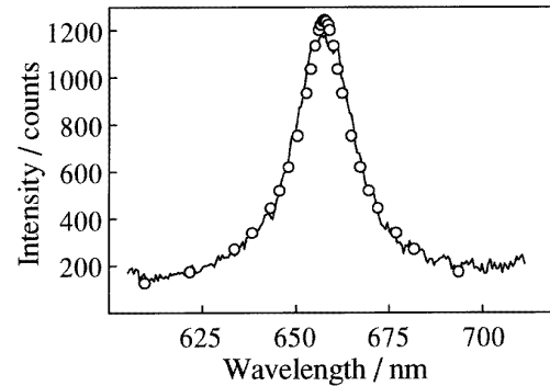
Figure 6. The H_\alpha line of positive streamers and a profile fit (circles). The fit yields N_e = 4 \times 10^{18} \text{ cm}^{-3} . Needle-plane electrodes were used, with U = +60 kV and gap distance 12 mm. Light was collected 4 mm from the needle.
