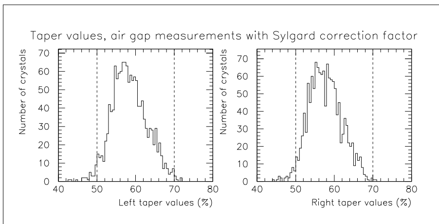
Figure 5.29: Left and right taper values, respectively, as measured with air gaps and converted to corresponding Sylgard taper values.
