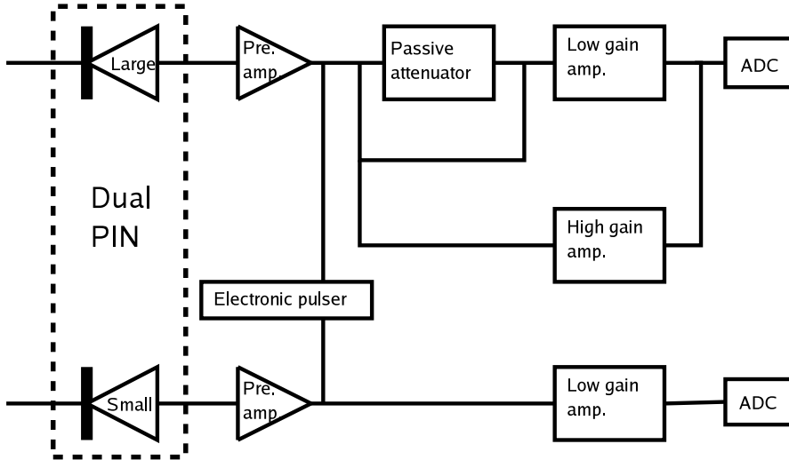
Figure 6.4: Schematics view of the readout options.
