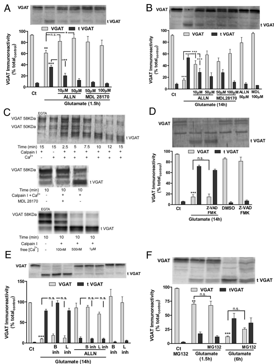
Figure 5. Calpain cleaves VGAT giving rise to tVGAT. A, B , Cultured hippocampal neurons were pre-incubated (2 h) with the calpain inhibitors MDL 28170 (50 and 100 \mu M) or ALLN (10 and 50 \mu M), before and during glutamate stimulation (125 \mu M, 20 min). The cells were then incubated in culture-conditioned medium for 1.5 h ( A ) or 14 h ( B ) with calpain inhibitors. The results are the average \pm SEM of at least five different experiments performed in independent preparations. C , Cerebrocortical synaptic vesicles (5 \mu g) were incubated with recombinant calpain I (2.5U/ml) for the indicated periods of time at 37°C, in the presence (100 nM, 500 nM, 1 \mu M, 2.5 mM \text{Ca}^{2+} ) or in the absence (1 mM EGTA) of calcium. Where indicated the effect of the calpain inhibitor MDL 28170 (50 \mu M) was tested. The results are representative of at least three independent experiments. D , The effect of the caspase inhibitor Z-VAD-FMK (50 \mu M) (and DMSO as vehicle) on glutamate-evoked VGAT cleavage was tested using the experimental conditions described in B . The effect of cathepsin B (Ca-074 Me, 50 \mu M) and L (Inhibitor III, 10 \mu M) inhibitors is shown in E . Cumulative inhibition of calpains (ALLN, 50 \mu M) and cathepsins was also tested in E . F shows experiments where the effect of the proteasome inhibitor MG132 (1 \mu M) on VGAT cleavage was tested. In the latter experiments the cells were preincubated for 30 min with the proteasome inhibitor before the glutamate stimulation. After excitotoxic stimulation, the cells were incubated in culture-conditioned medium in the presence or in the absence of the tested inhibitor, for the indicated periods of time. In all experiments the extracts were analyzed by Western blot with an antibody against VGAT. In the results of D–F the average \pm SEM of at least four experiments was performed in independent preparations. Statistical analysis was performed using one-way ANOVA followed by Bonferroni's multiple comparison test. * p < 0.05 , ** p < 0.01 , *** p < 0.001 ; n.s., not significant, compared with the control protein levels for VGAT or tVGAT or for the indicated comparisons.
