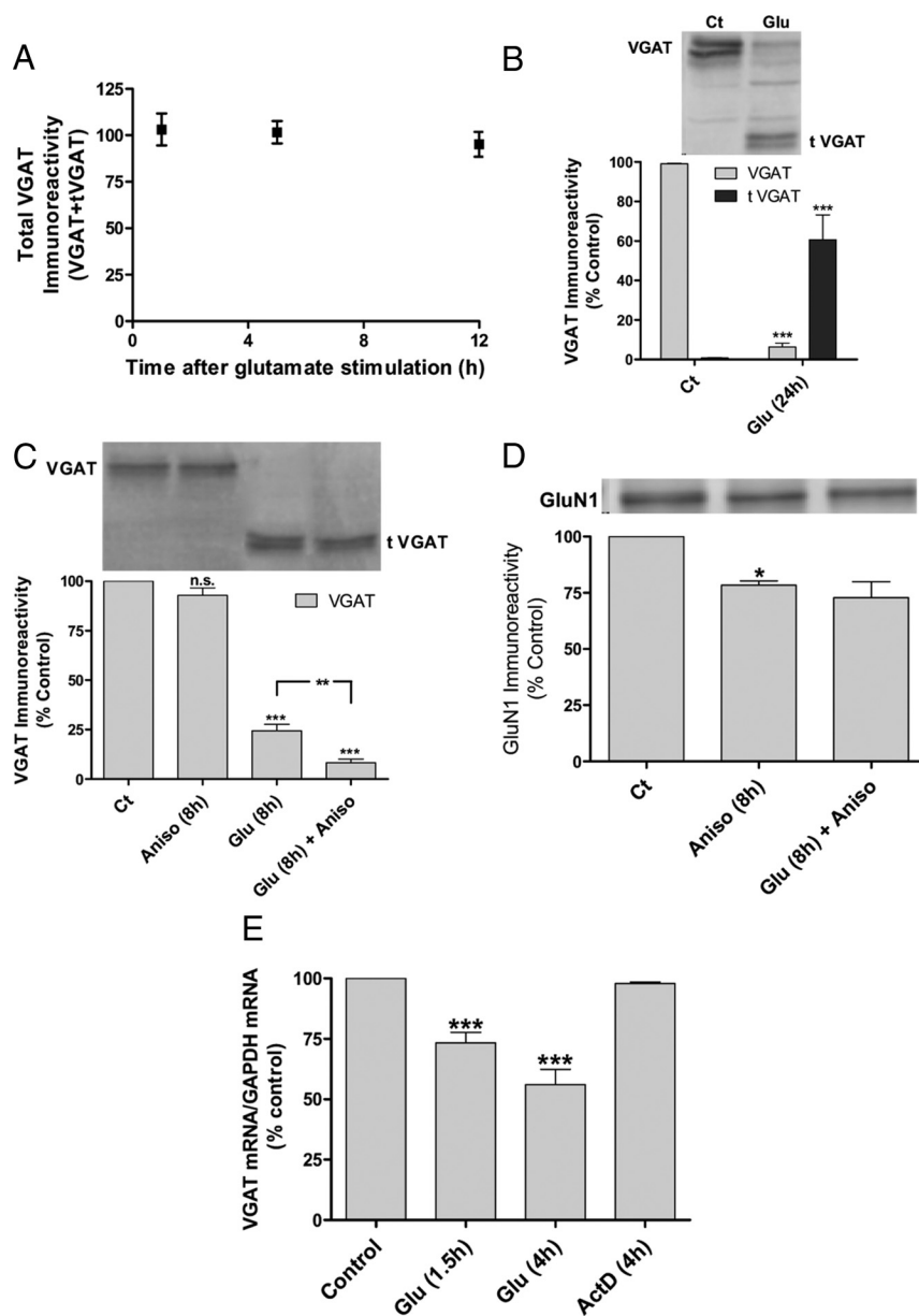
Figure 4. tVGAT has a long half-life. A–C , Cultured hippocampal neurons were subjected to excitotoxic stimulation with glutamate (125 \mu\text{M} glutamate, 20 min) and further incubated in culture-conditioned medium for the indicated period of time. VGAT and tVGAT protein levels were determined by Western blot. The results are the average \pm SEM of 4 ( A , B , D , E ) or 4–12 ( C ) independent experiments, performed in different preparations (in A the results were taken from Fig. 1A). Where indicated the cells were stimulated in the presence or in the absence of the protein synthesis inhibitor anisomycin (5 \mu\text{M} ), and were further incubated in culture-conditioned medium for 8 h, in the presence or in the absence of the translation inhibitor. E , Cultured hippocampal neurons were subjected to excitotoxic stimulation with glutamate (125 \mu\text{M} glutamate, 20 min) and further incubated in culture-conditioned medium for the indicated periods of time. Alternatively, cultures were incubated with the transcription inhibitor actinomycin D (1.5 \mu\text{M} ) for 4 h. Total RNA was extracted and VGAT and Gapdh mRNA were semiquantified through real-time PCR. Statistical analysis was performed using one-way ANOVA followed by Dunnett's ( A ) or Bonferroni's ( B–E ) multiple comparison tests. * p < 0.05 , *** p < 0.001 , compared with the control; ** p < 0.01 for the indicated comparison; n.s., not significant.
