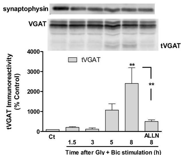
Figure 3. VGAT is cleaved under conditions that induce chemical LTP. Cultured hippocampal neurons (15 DIV) were stimulated with 0.2 mM glycine and 0.01 mM bicuculline for 15 min in ACSF. The cells were then incubated in culture-conditioned medium for the indicated periods of time before preparation of the extracts. Where indicated, the cells were pre-incubated with the calpain inhibitor ALLN (50 \mu M) for 2 h, and the inhibitor was also present in the culture-conditioned medium after excitotoxic stimulation. The results were analyzed by Western blot, using an antibody against VGAT. The results are the average \pm SEM of three different experiments performed in independent preparations. Statistical analysis was performed using the one-way ANOVA followed by Newman–Keuls multiple comparison test. ^{**}p < 0.01 , compared with the control or with cells exposed to chemical LTP in the absence of ALLN.
